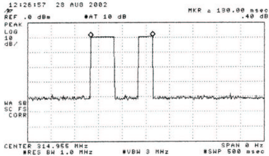
Figure 6.4. Transmitter 5 sec. transmission limit verification
