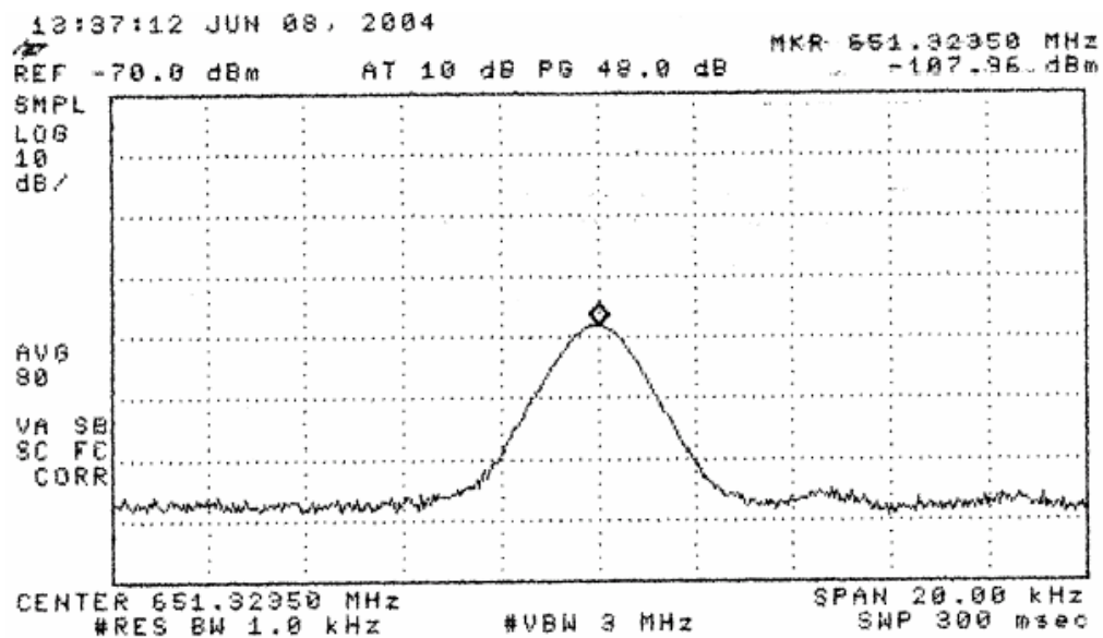
Figure 6.1. Relative receiver emissions in activated mode.
