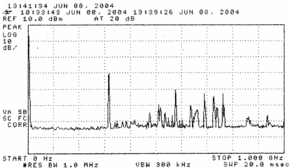
Figure 5.1. Emissions measured at 3 meters in anechoic chamber, 0-1000 MHz. (top) Receiver plus ambient (bottom) Ambient
