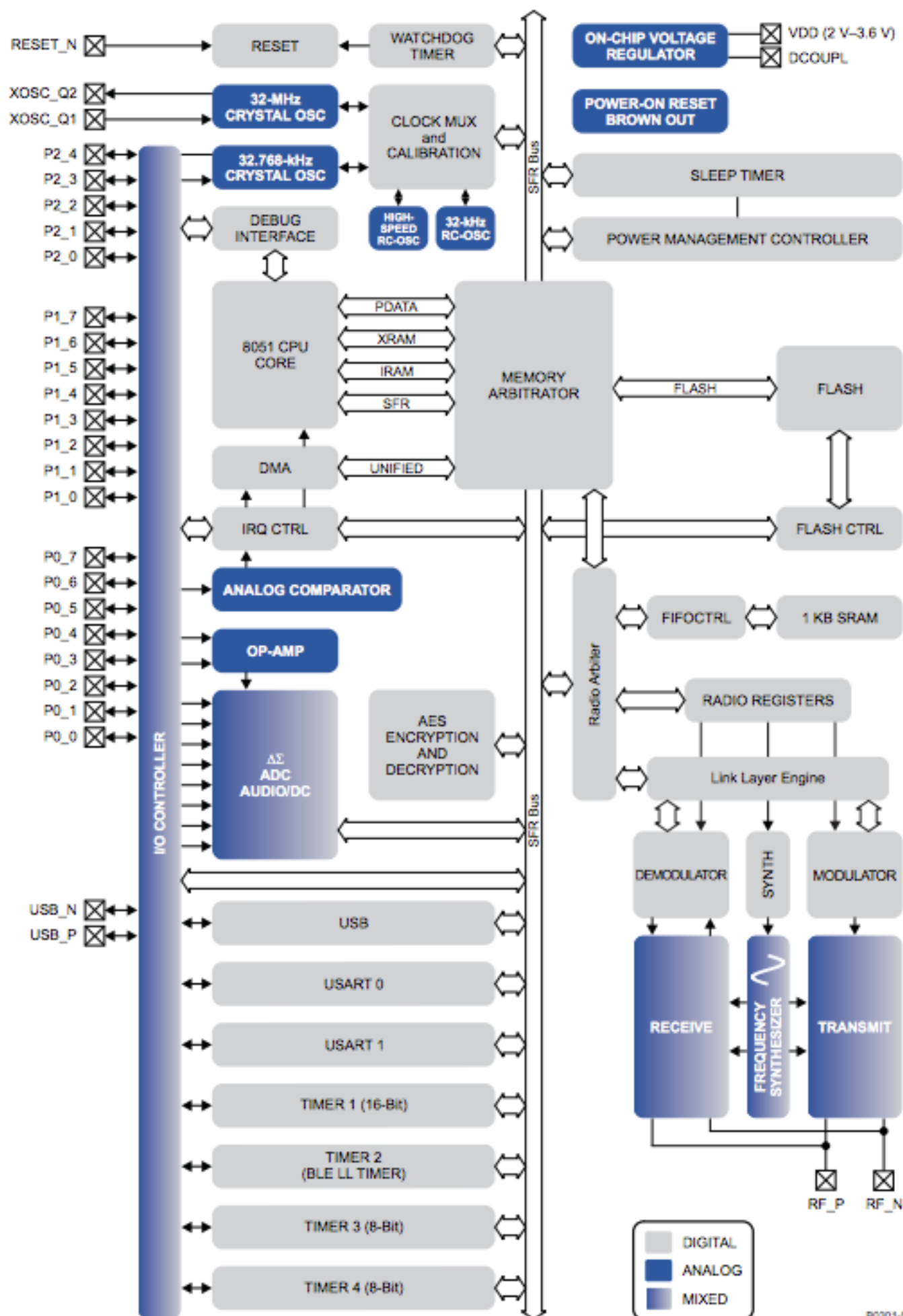
Figure 8. CC2540 Block Diagram
