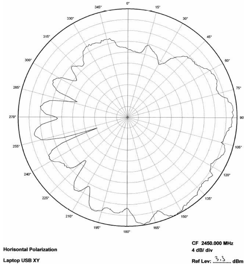
Figure 14: USB Dongle in Laptop XY Plane
