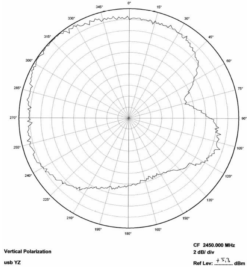
Figure 11: USB Dongle YZ Plane
