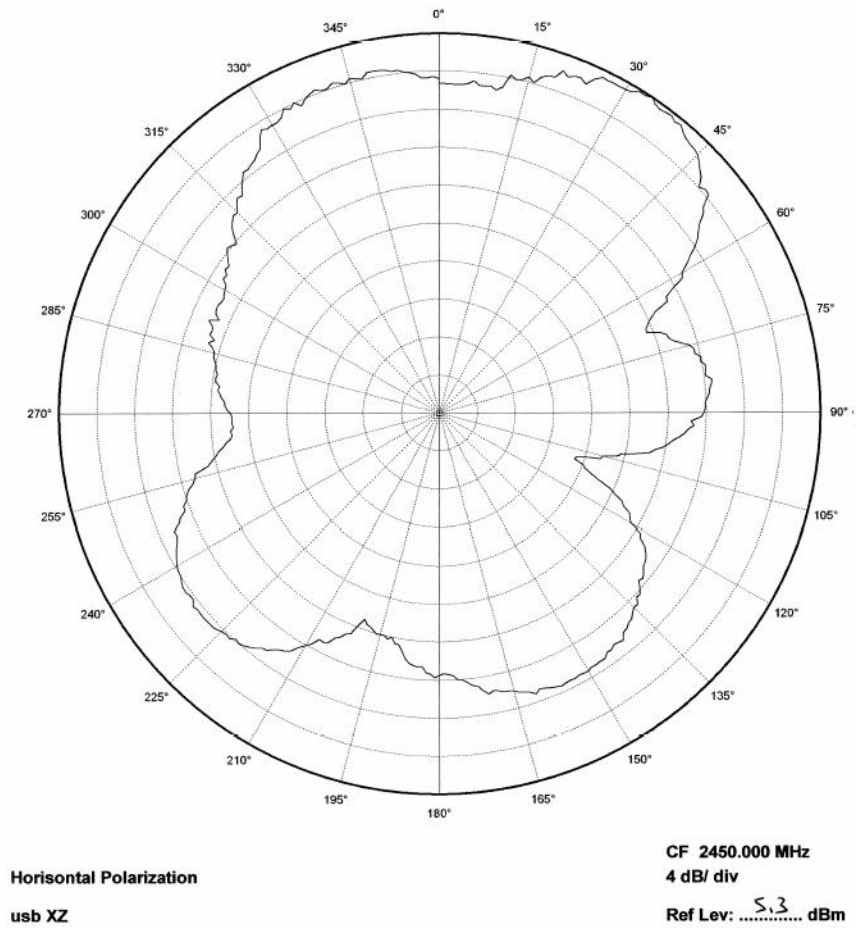
Figure 10: USB Dongle XZ Plane
