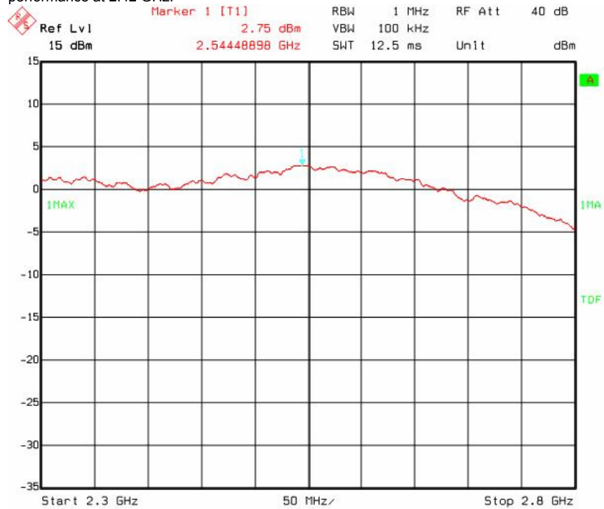
Figure 15: Output Power, USB Dongle
