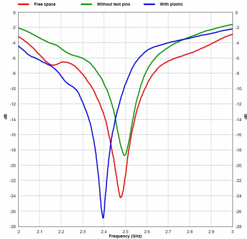
Figure 4: Influence of Plastic Encapsulation and Test Pins
