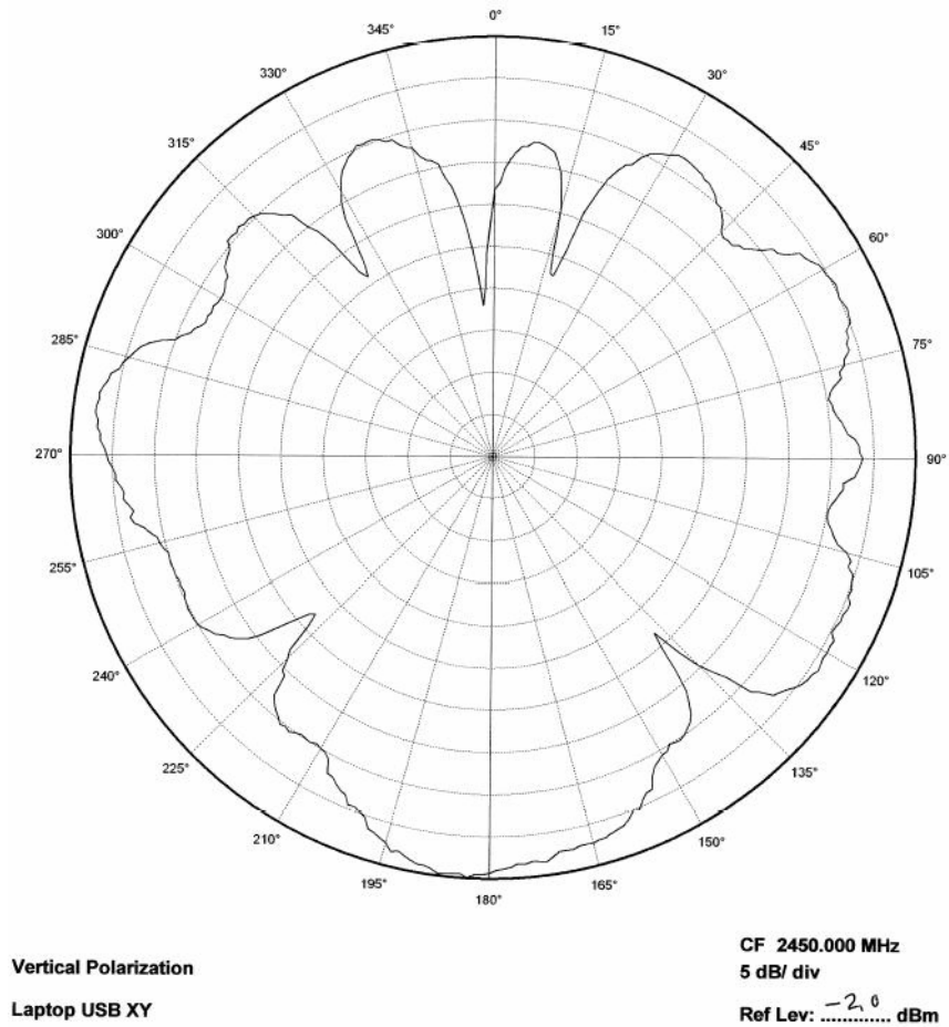
Figure 13: USB Dongle in Laptop XY Plane
