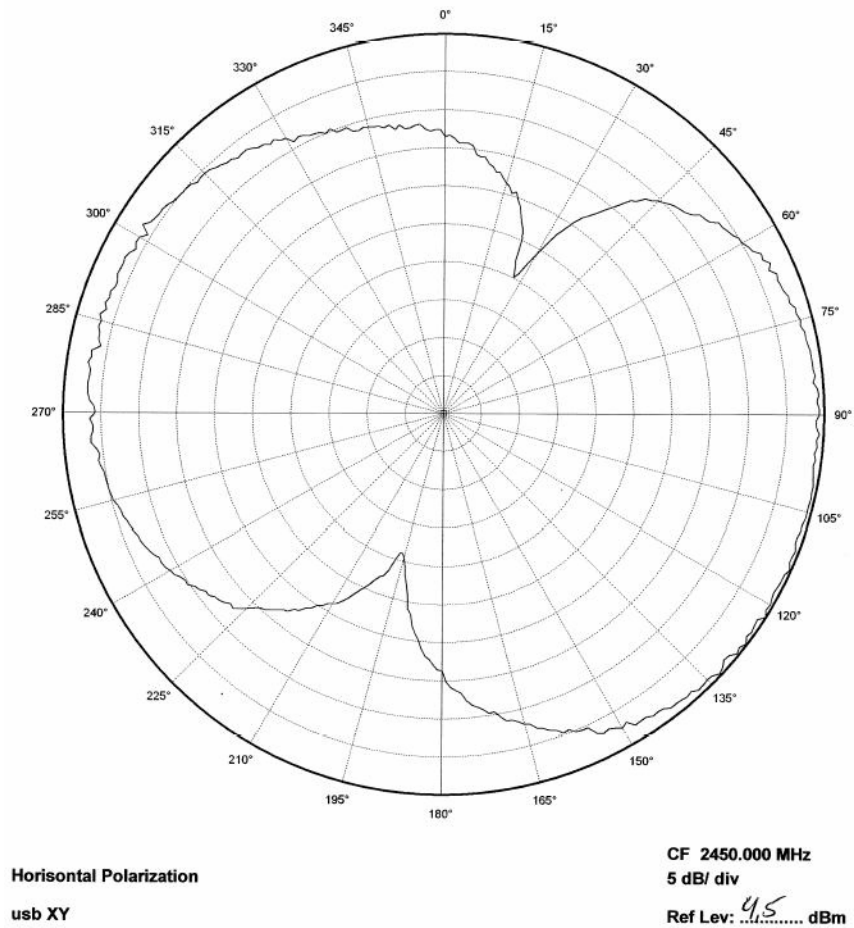
Figure 8: USB Dongle XY Plane
