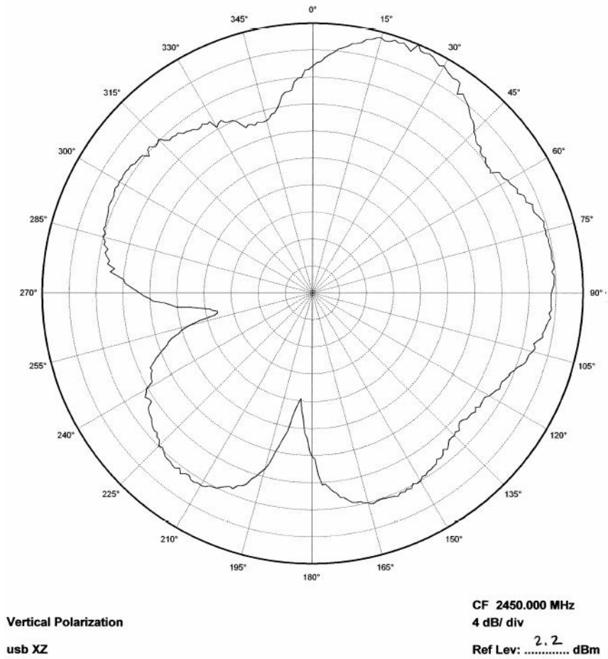
Figure 9: USB Dongle XZ Plane
