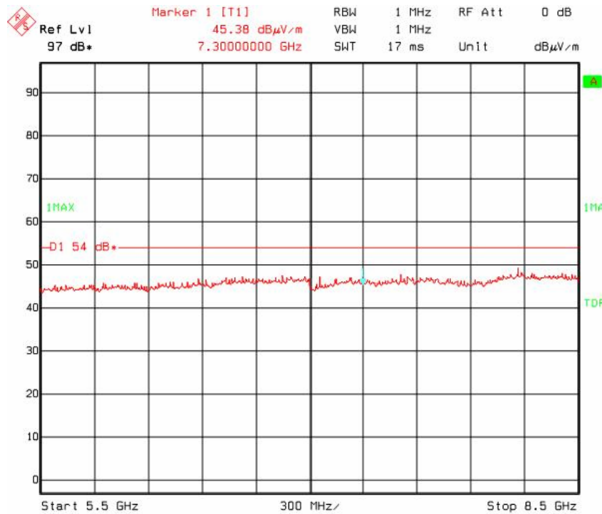
Figure 18: TX Spurious Emission 5.5 – 8.5 GHz
