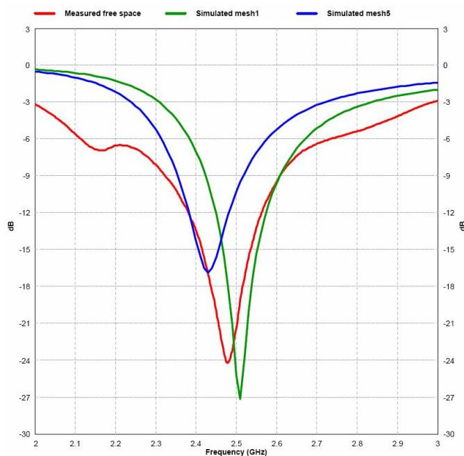
Figure 2: Comparison of Simulation and Measurements Results
