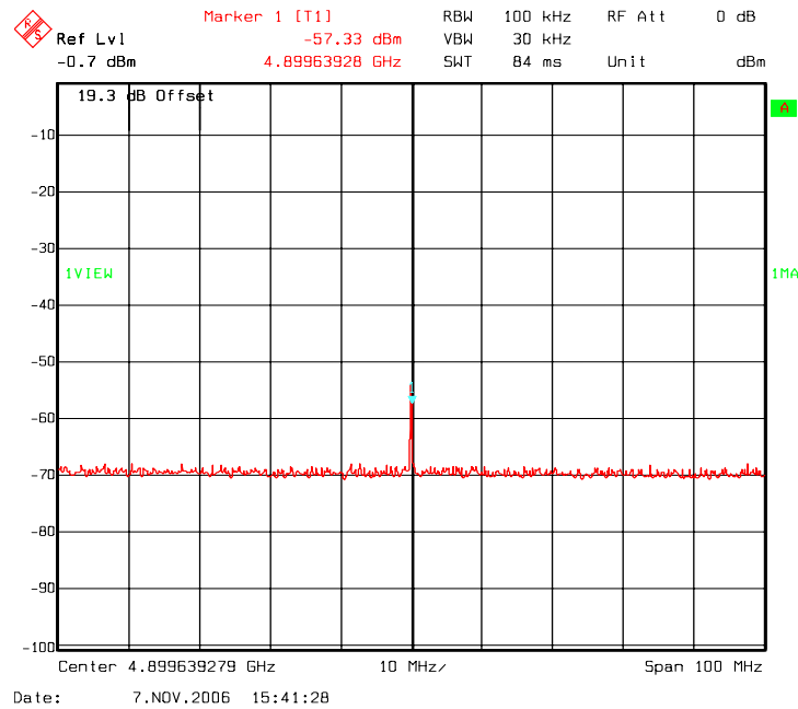
Figure 19: RX Spurious Emission
