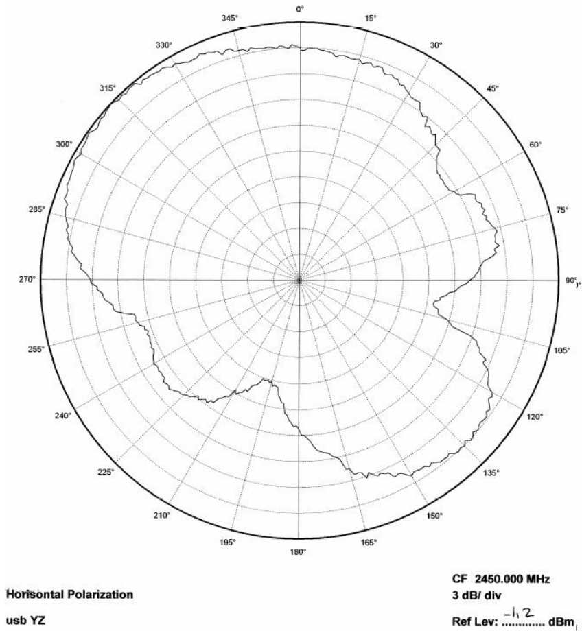
Figure 12: USB Dongle YZ Plane
