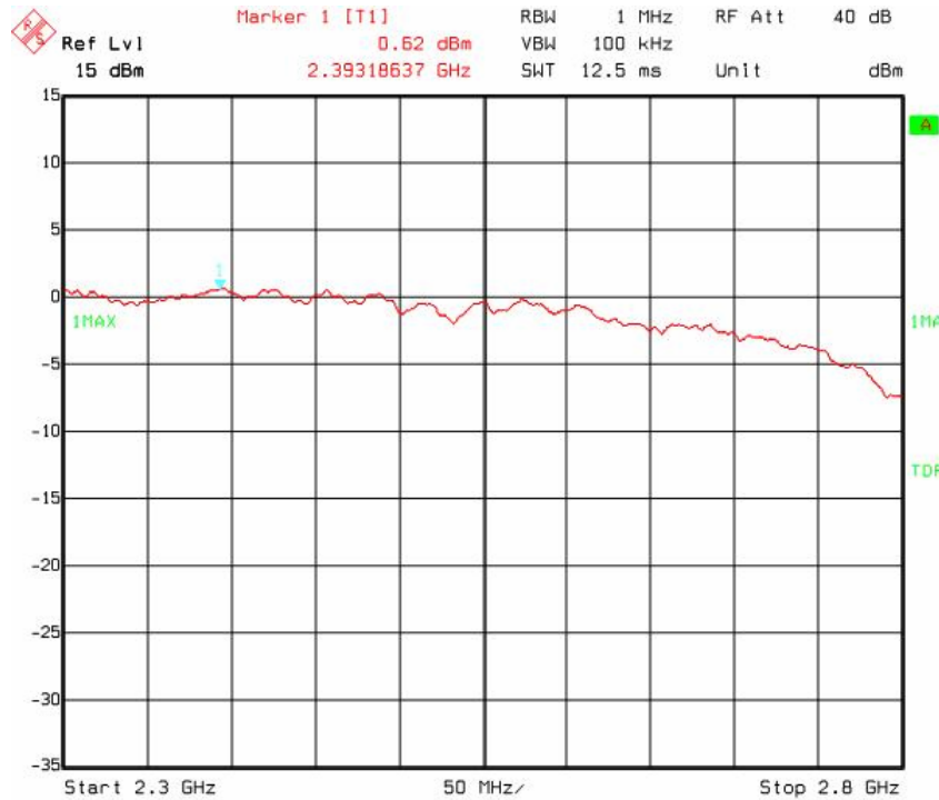
Figure 16: Output Power, USB Dongle in Laptop
