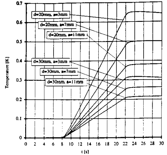
Fig. 5. Temperature increase measured during RF exposure to a 900 MHz field. The power input was 43 dBm. d = dipole distance from the simulating liquid; a = sensor distance from the acrylic glass bottom.
