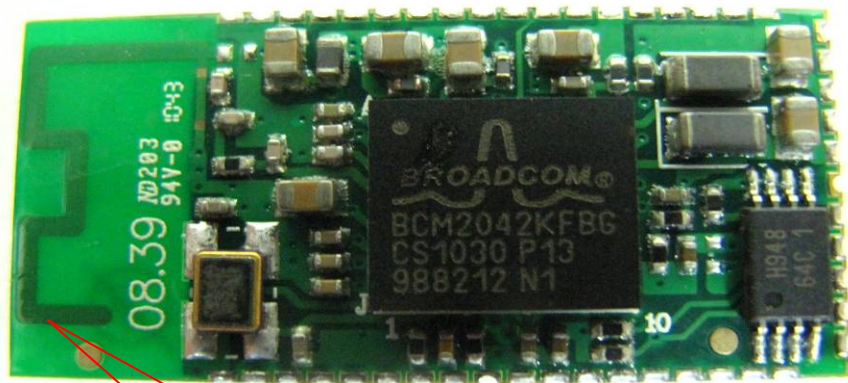
BT Antenna
