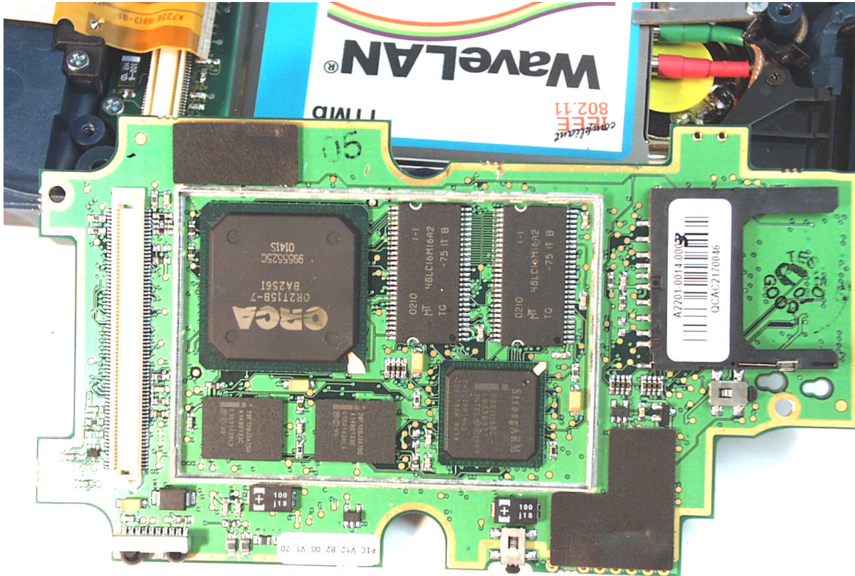
ANNEX 4 - INTERNAL PHOTOGRAPHS OF EUT NETPAD + TRX7431 (DSSS Modular Transceiver), Model NETPAD RLAN
