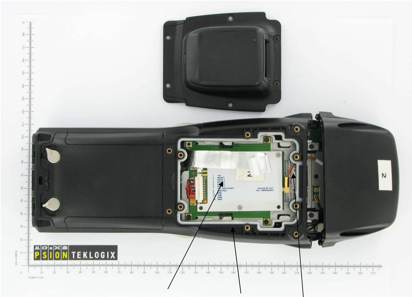
RFID Module on XMOD Bluetooth on the Main logic board (native on the WAP) WIFI RA2041 on the CF-card slot
