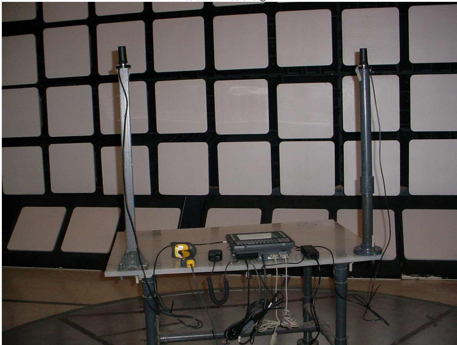
Radiated Emissions @ 3 m
