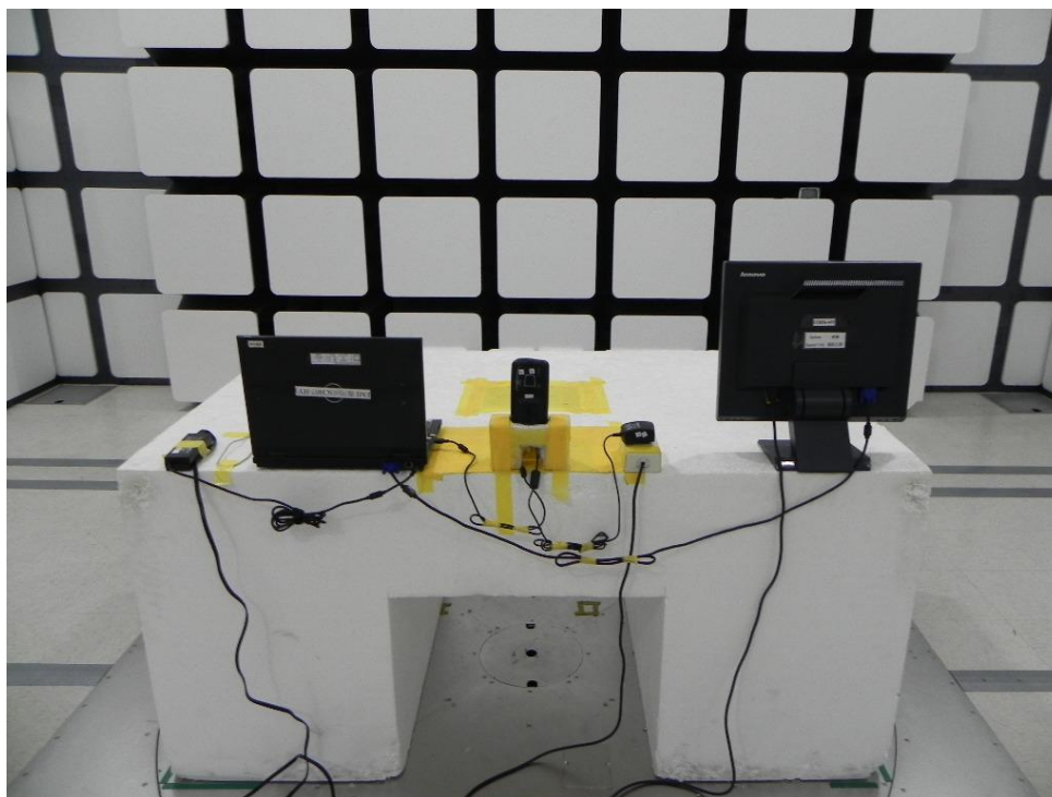
<Rear View>
