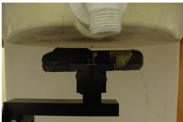
Front Face of the DUT with Phantom 1.5 cm Gap (DUT with Charger Snap Module 2)
