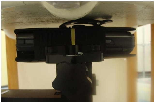
Front Face of the DUT and Holster with Phantom 0 cm Gap
