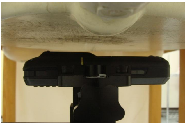
Rear Face of the DUT with Phantom 1.5 cm Gap
