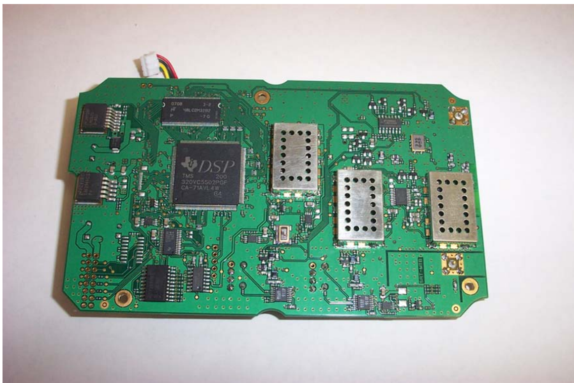
Figure 3: OEM PCB bottom side
