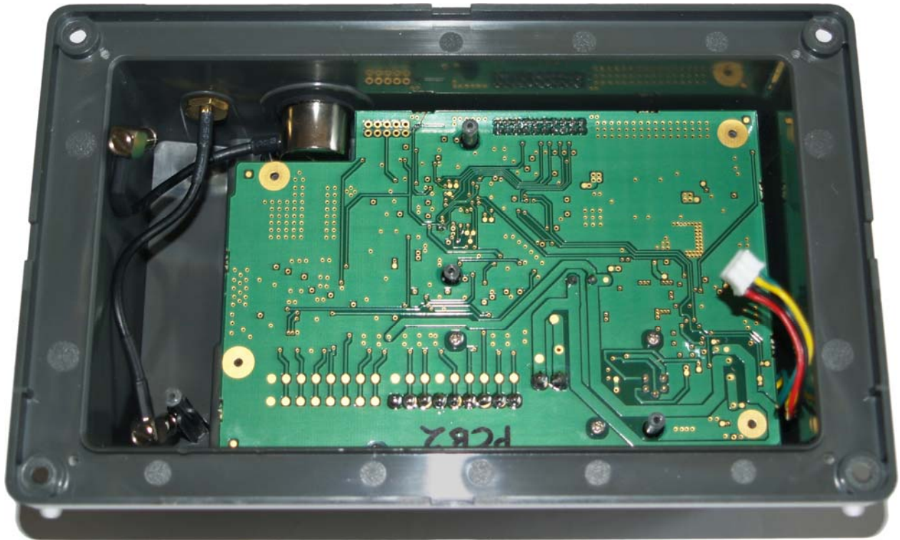
Figure 6: Internal view showing Interface PCB
