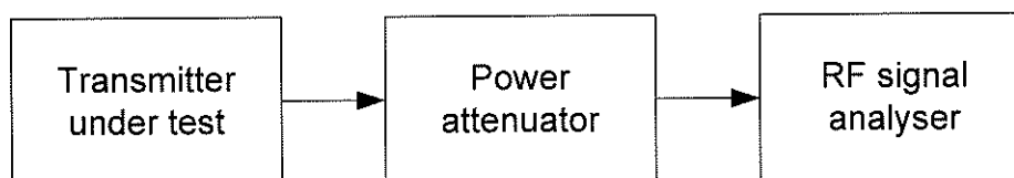
Figure 2 Measurement arrangement for modulation accuracy
