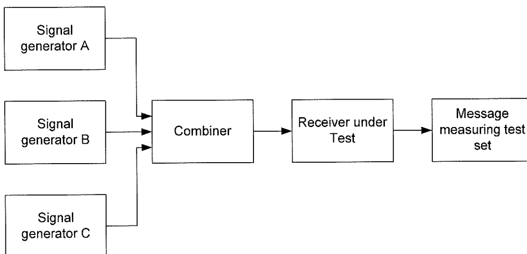
Figure 6 Measurement arrangement for intermodulation
