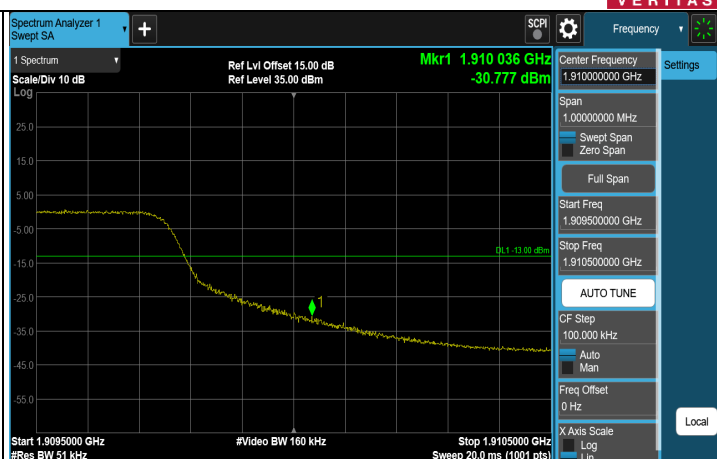
256QAM FULL CH 19175 (1907.5 MHz)
