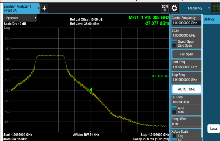
256QAM 1RB CH 19193 (1909.3 MHz)
