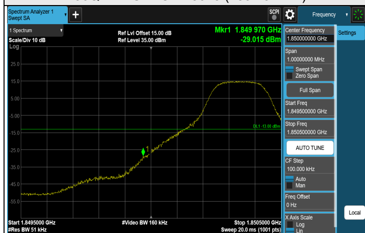
256QAM 1RB CH 18625 (1852.5 MHz)
