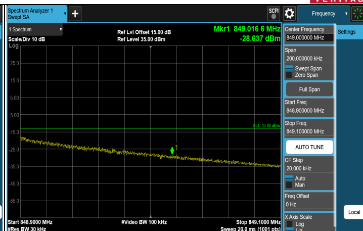
256QAM FULL CH 20635 (847.5 MHz)
