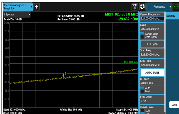
256QAM FULL CH 20415 (825.5 MHz)
