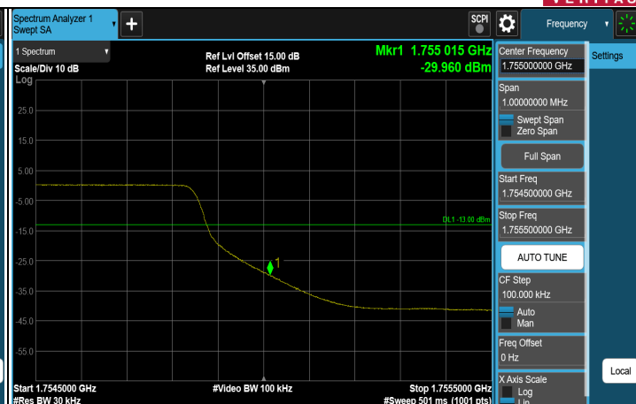
256QAM FULL CH 20385 (1753.5 MHz)
