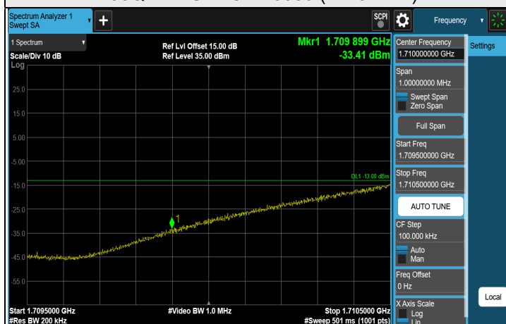
256QAM 1RB CH 20050 (1720 MHz)
