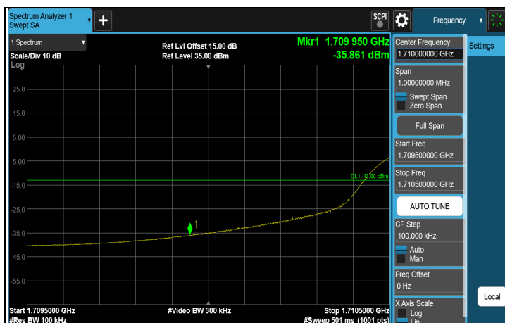
256QAM FULL CH 20000 (1715 MHz)
