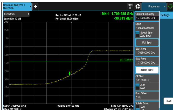
256QAM FULL CH 19965 (1711.5 MHz)
