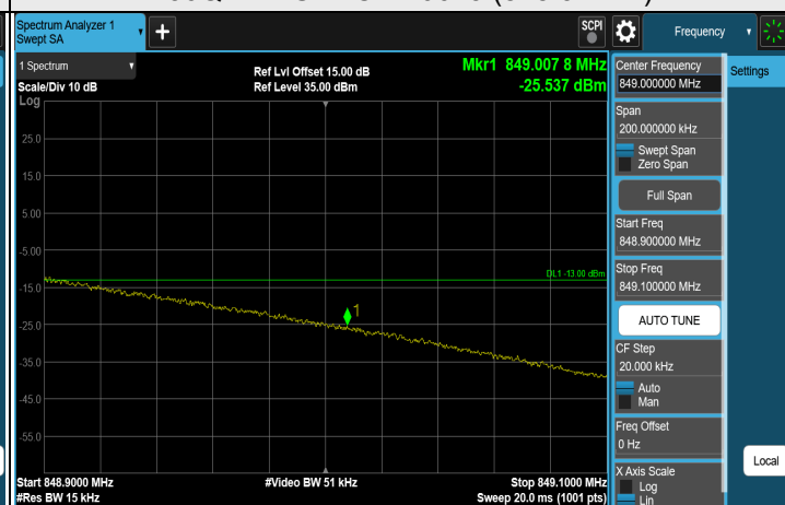
256QAM 1RB CH 20643 (848.3 MHz)
