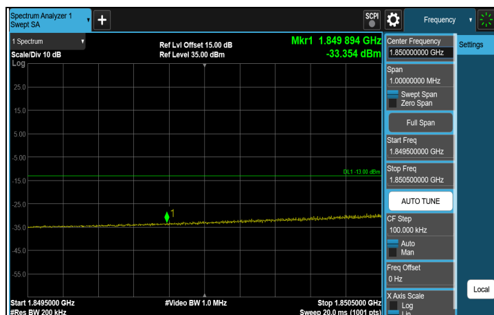
256QAM FULL CH 18700 (1860 MHz)
