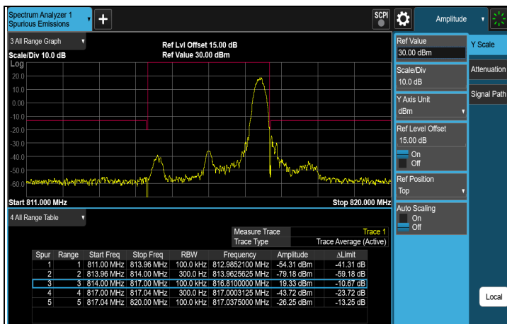
256QAM 1RB#MAX CH 26705 (815.5 MHz)
