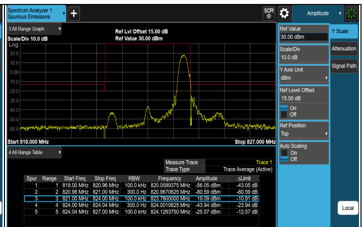
256QAM 1RB#MAX CH 26775 (822.5 MHz)
