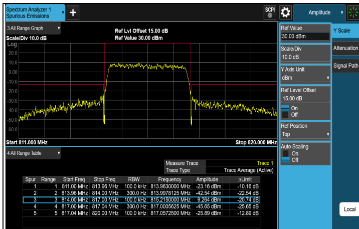
256QAM FULL CH 26705 (815.5 MHz)
