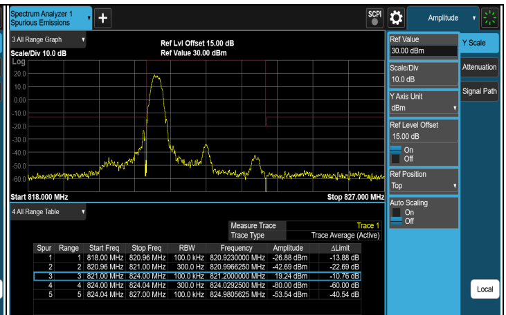
256QAM 1RB#0 CH 26740 (819 MHz)
