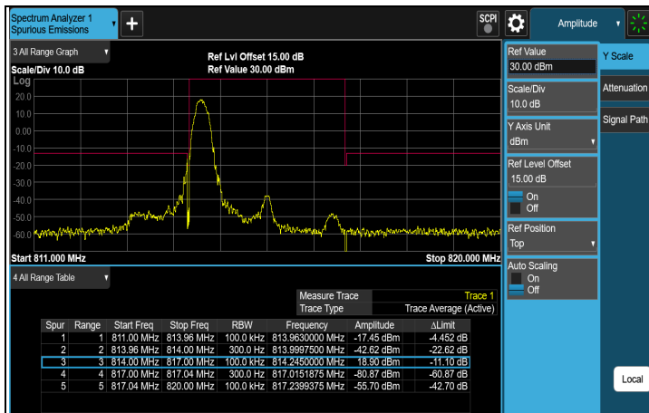
256QAM 1RB#0 CH 26705 (815.5 MHz)
