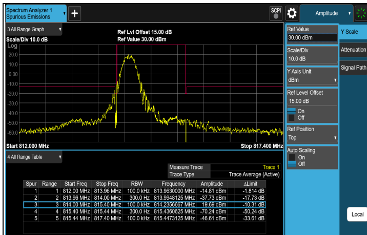
256QAM 1RB#0 CH 26697 (814.7 MHz)
