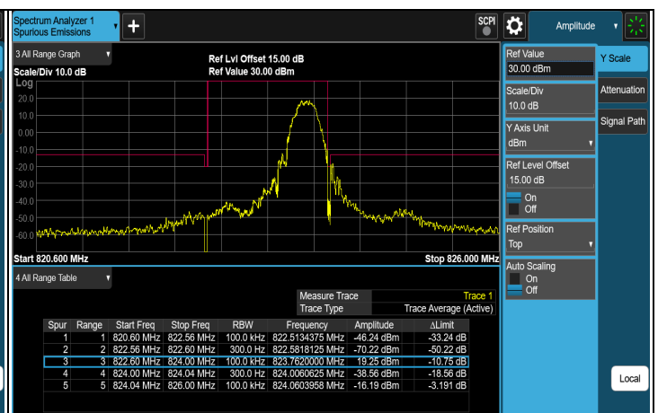
256QAM 1RB#MAX CH 26783 (823.3 MHz)
