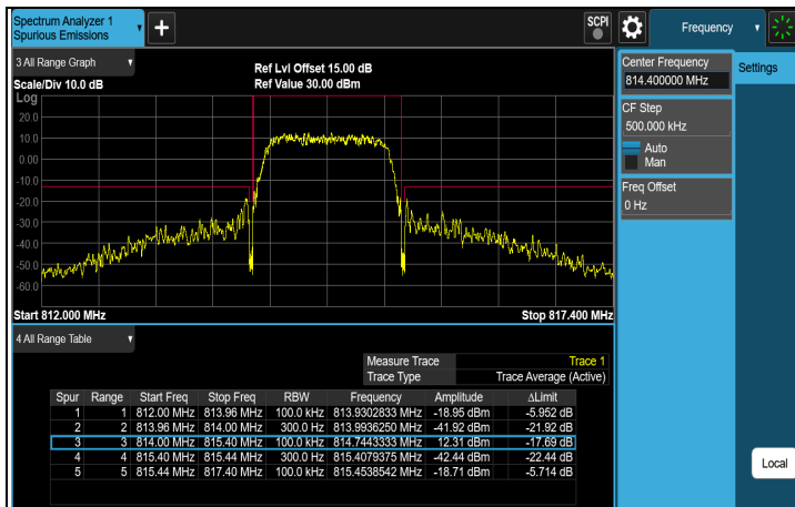
256QAM FULL CH 26697 (814.7 MHz)
