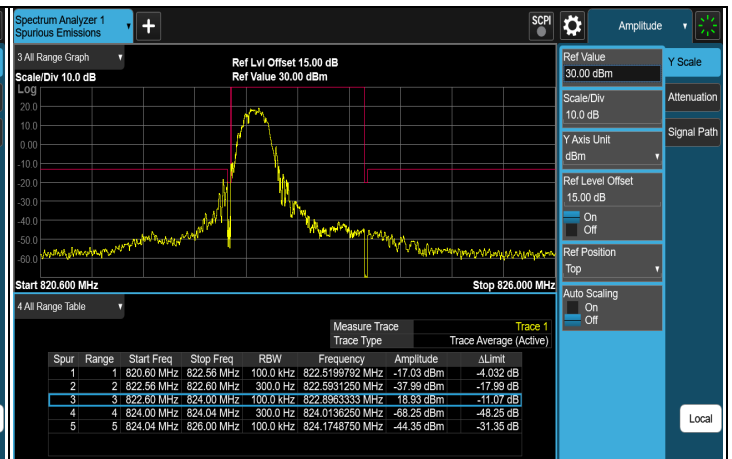
256QAM 1RB#0 CH 26783 (823.3 MHz)
