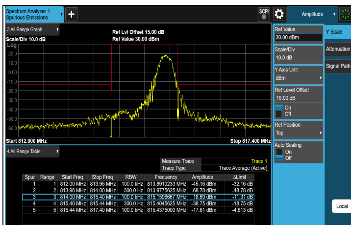
256QAM 1RB#MAX CH 26697 (814.7 MHz)
