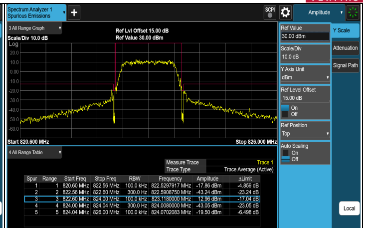
256QAM FULL CH 26783 (823.3 MHz)
