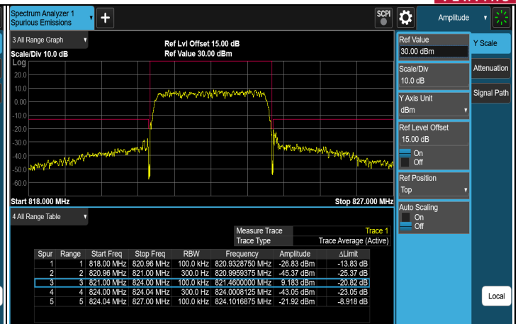
256QAM FULL CH 26740 (819 MHz)
