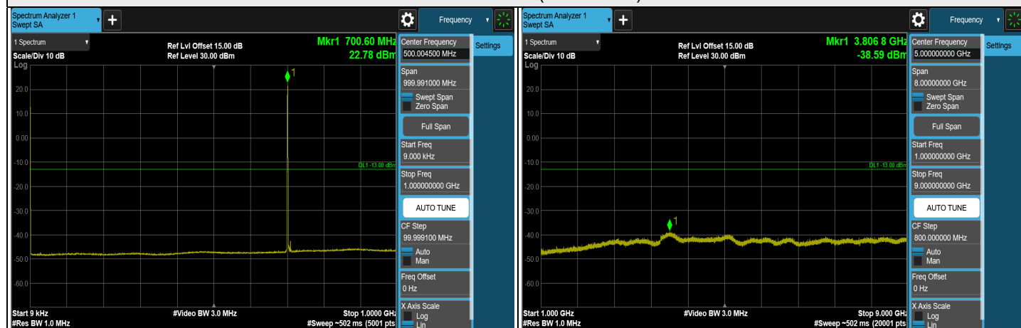
Channel 141500 (707.5 MHz)
