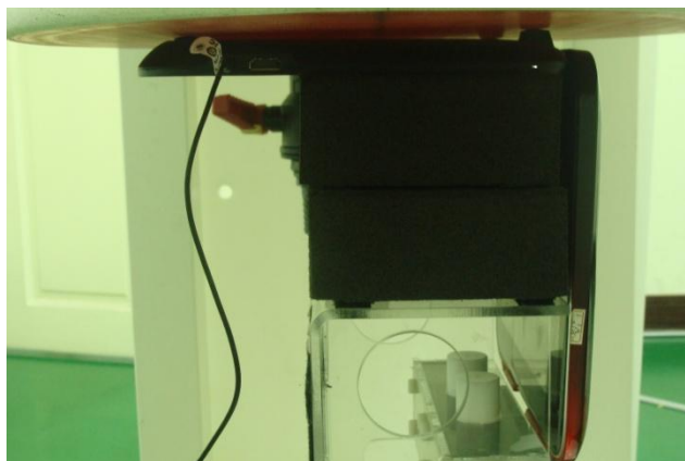
Bottom of DUT with Phantom 0 cm Gap
