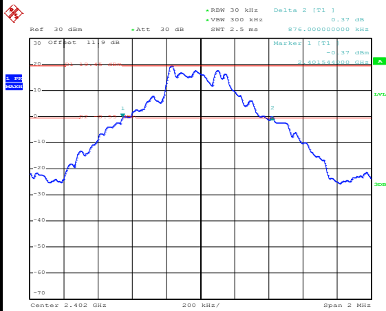
20 dB Bandwidth Plot on Channel 00
