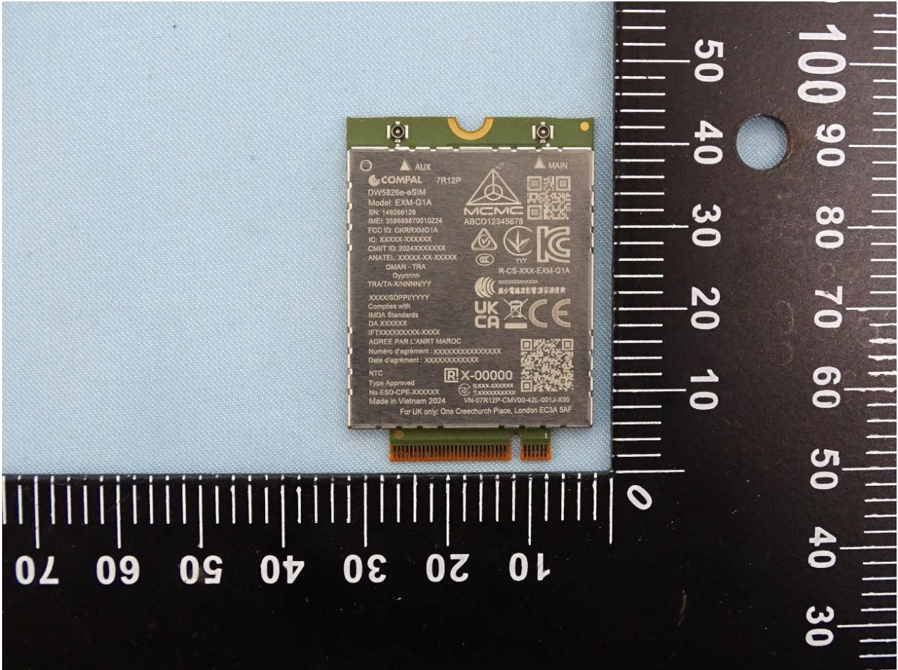
LTE Module (Brand Name: COMPAL/ Model Name: EXM-G1A)
