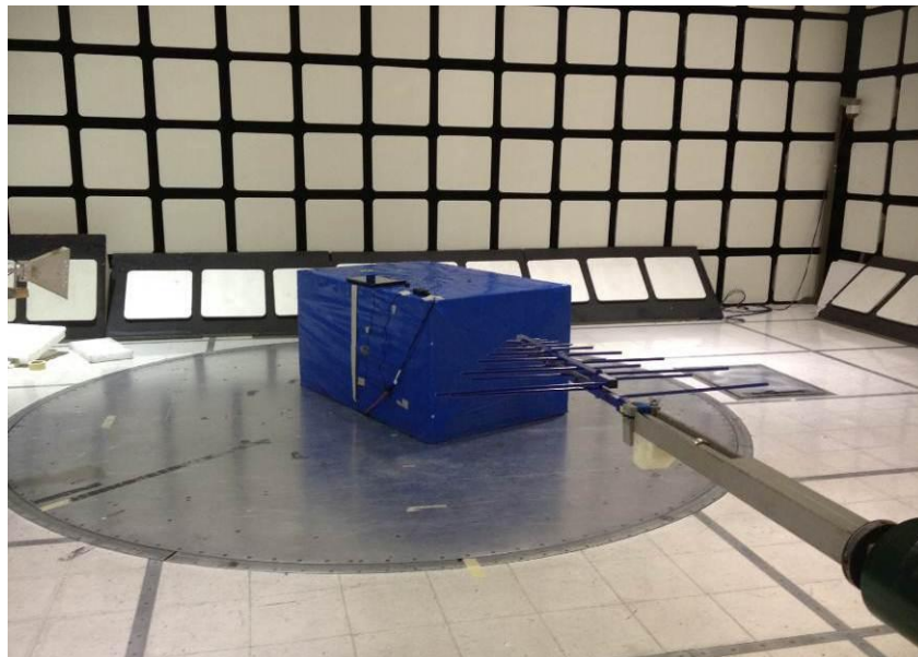
Test Setup
