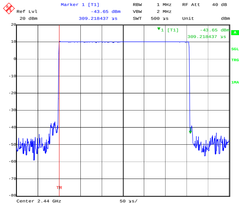
Dwell Time, GFSK (Single Pulse)
