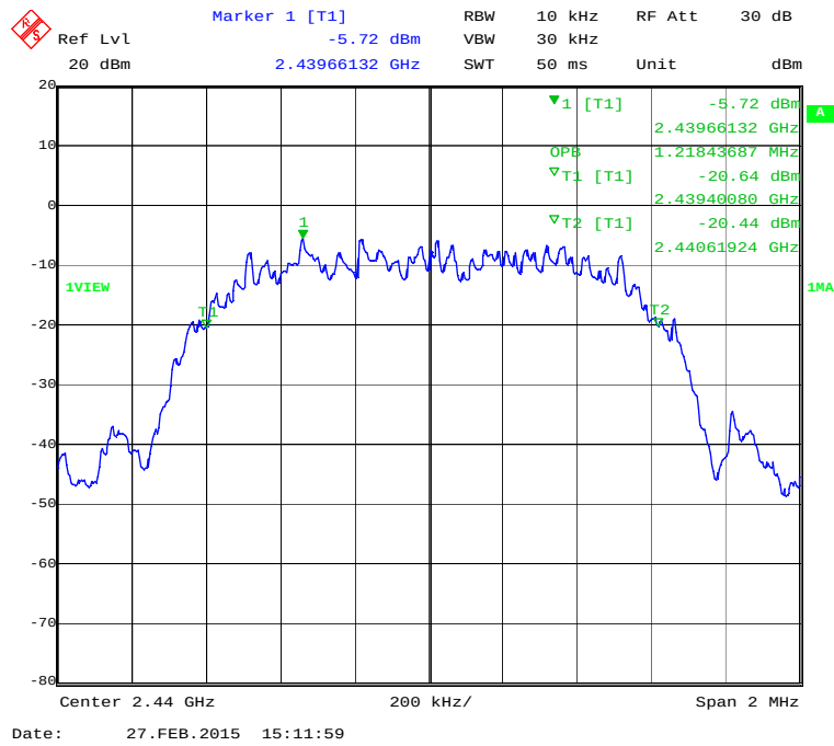
99% Bandwidth, EDR2
