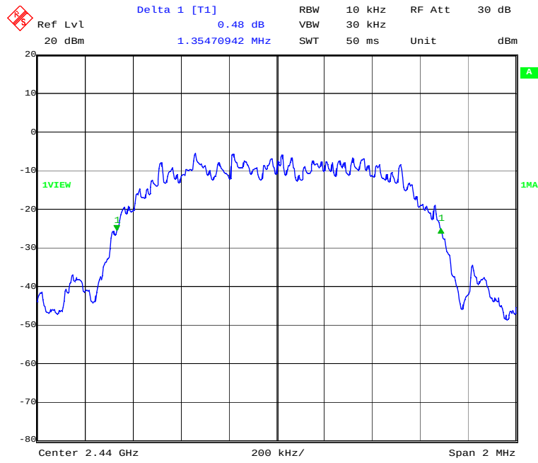
20dB Bandwidth, EDR2
