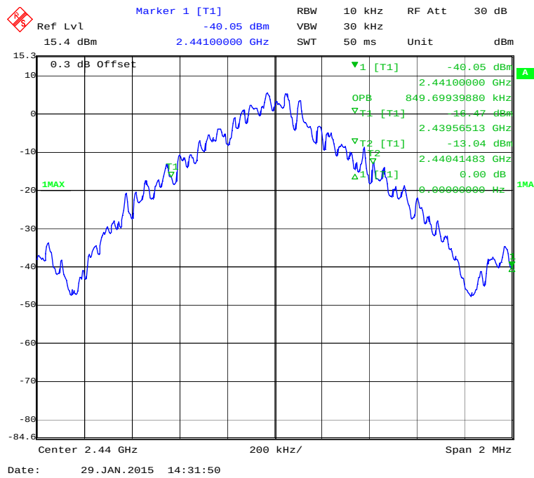
99% Bandwidth, GFSK
