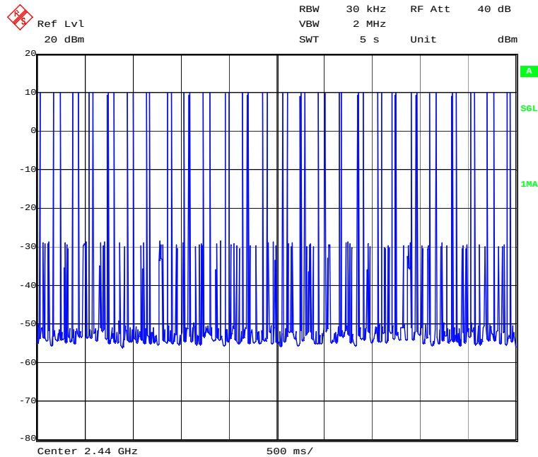
Dwell Time, GFSK
