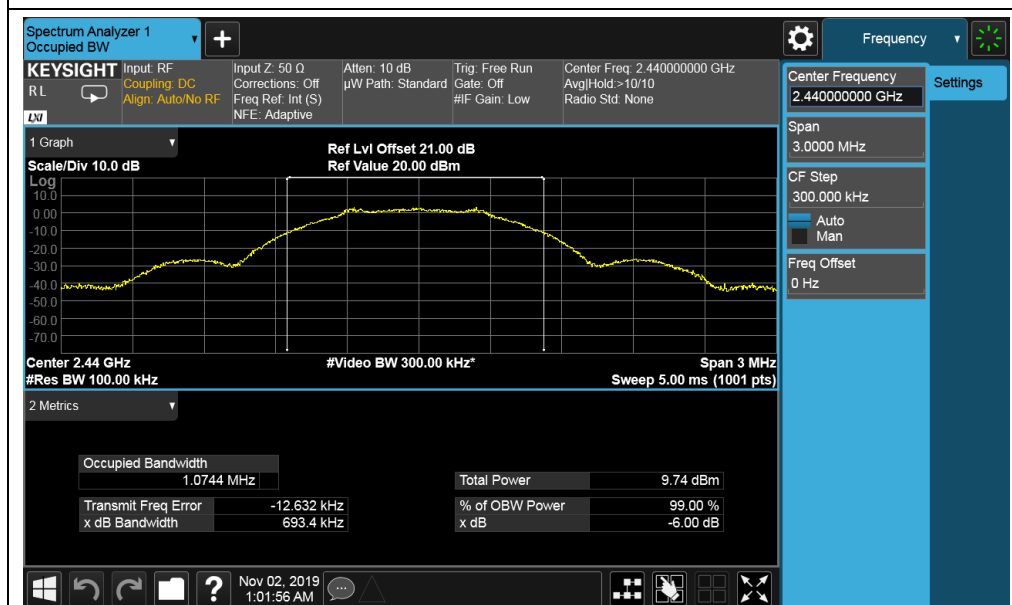
BLE-2440MHz
