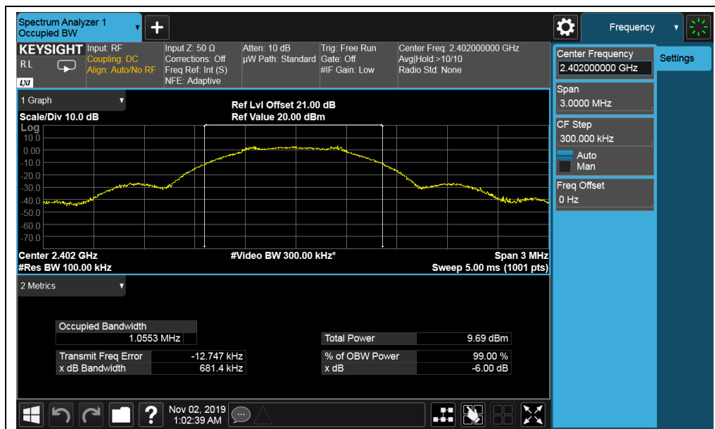
BLE-2402MHz
