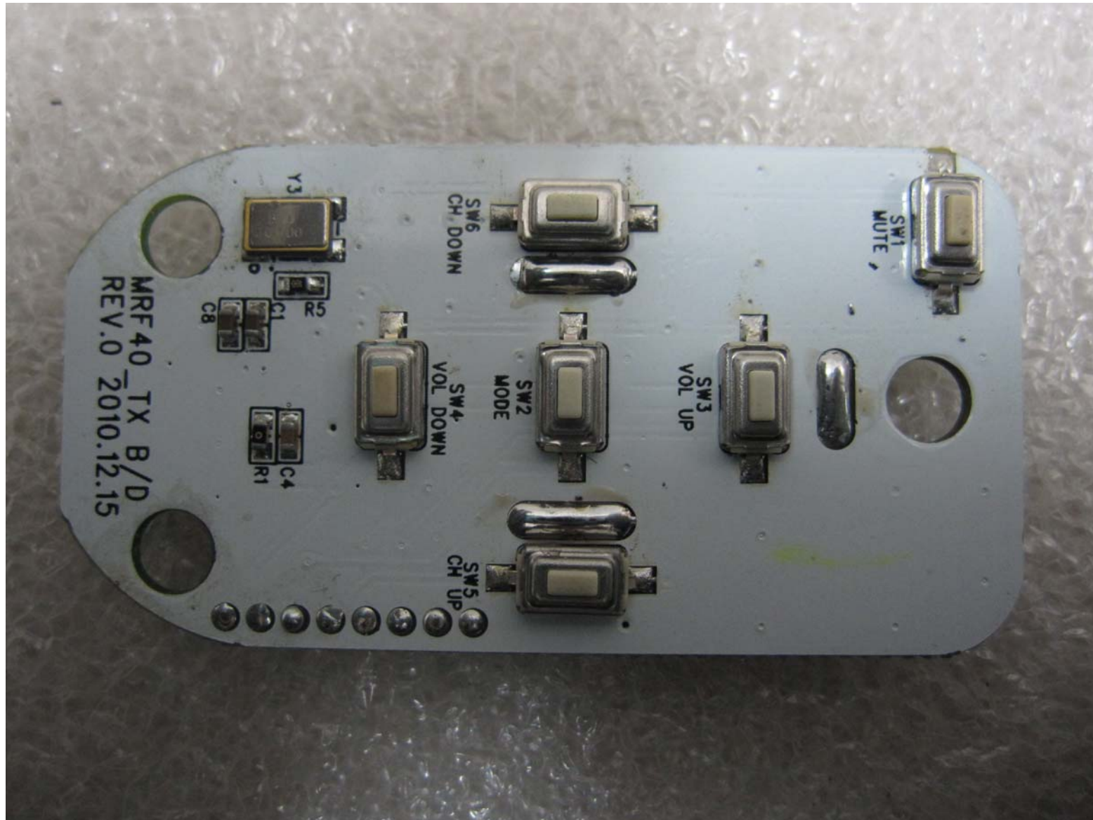
RF30(Remote)_Front of Main Board
