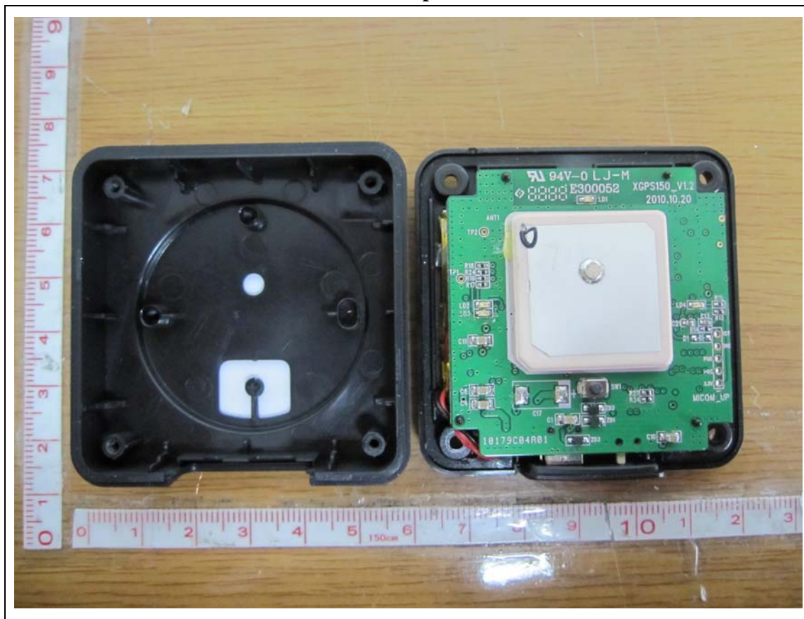
Internal photo
