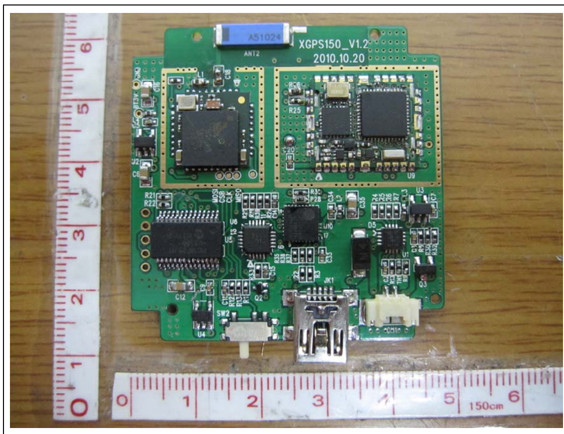
MainBoard - Rear
