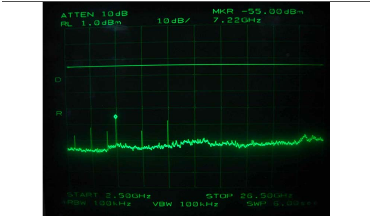
Low Channel
