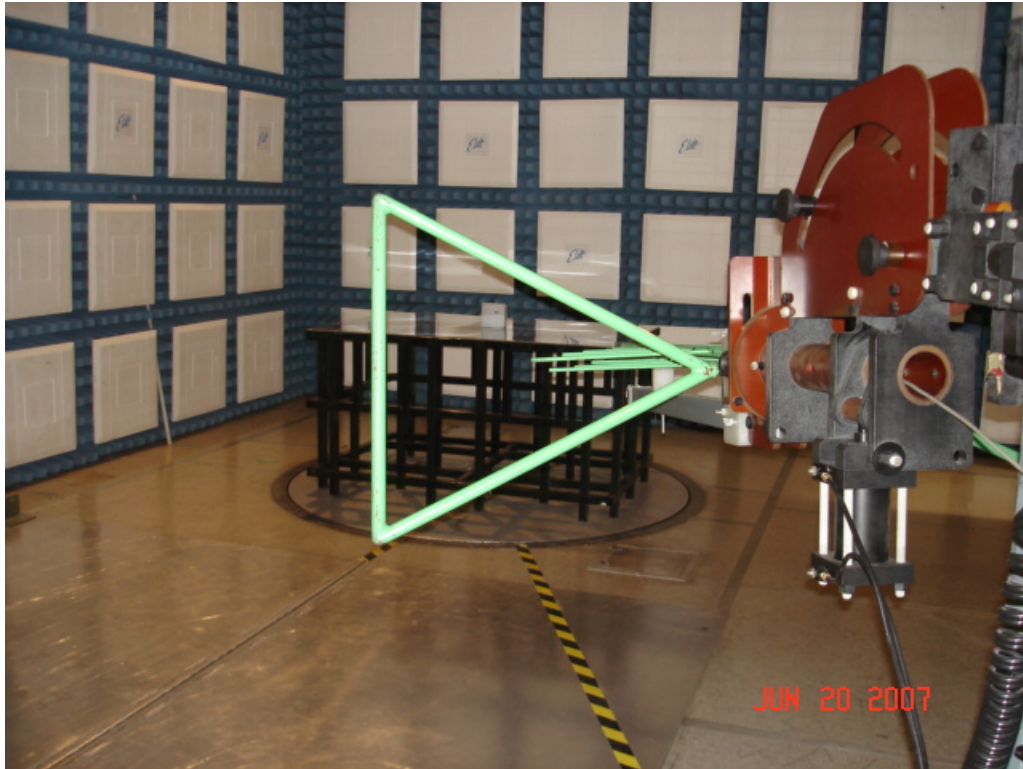
Test Setup for Radiated Emissions, 30MHz to 1GHz, Receiver – Horizontal Polarization
