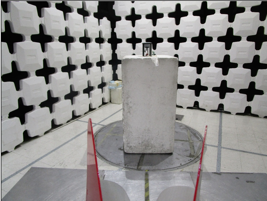
Test Setup for Spurious Emissions: Horizontal Polarization
