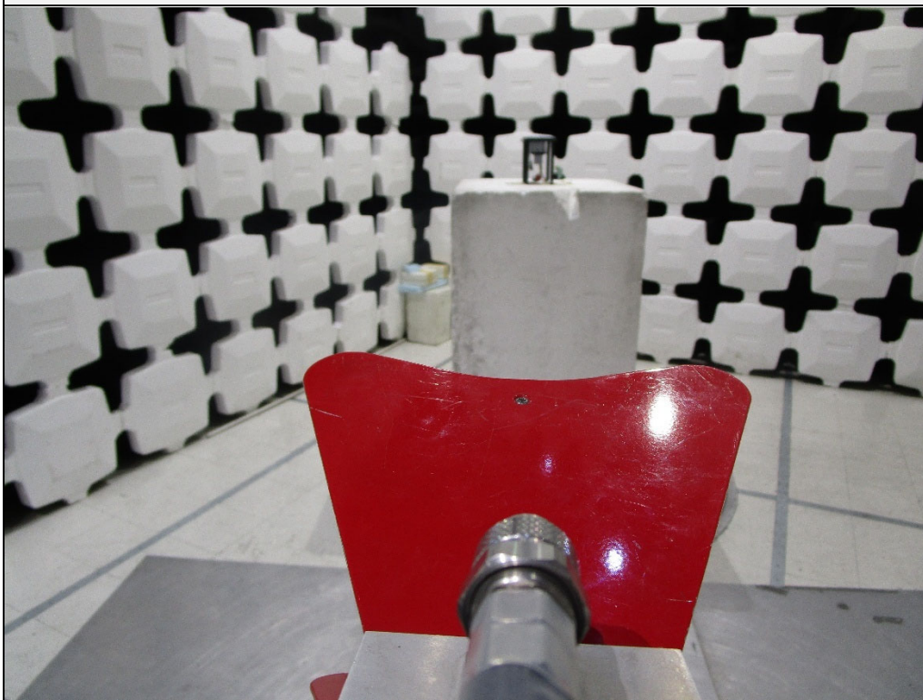
Test Setup for Spurious Emissions: Vertical Polarization
