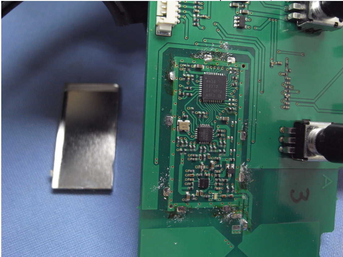
Figure 7 Internal View (RF Module, Removed Metal Cover)
