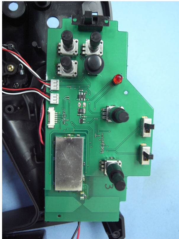
Figure 6 Internal View (Main Board, Front View)
