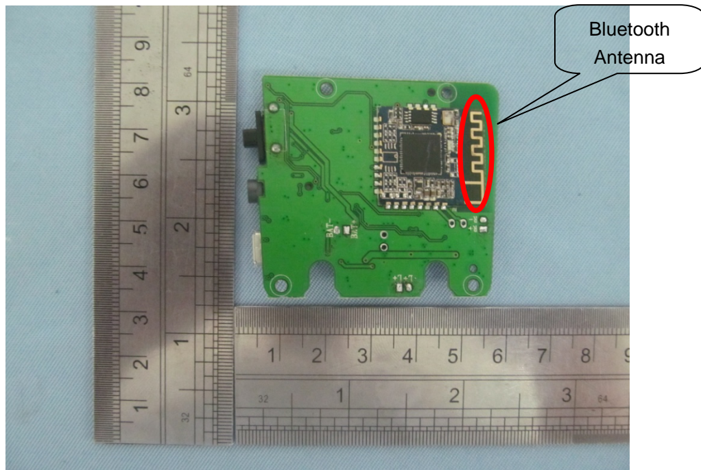
BACK VIEW OF PCB
