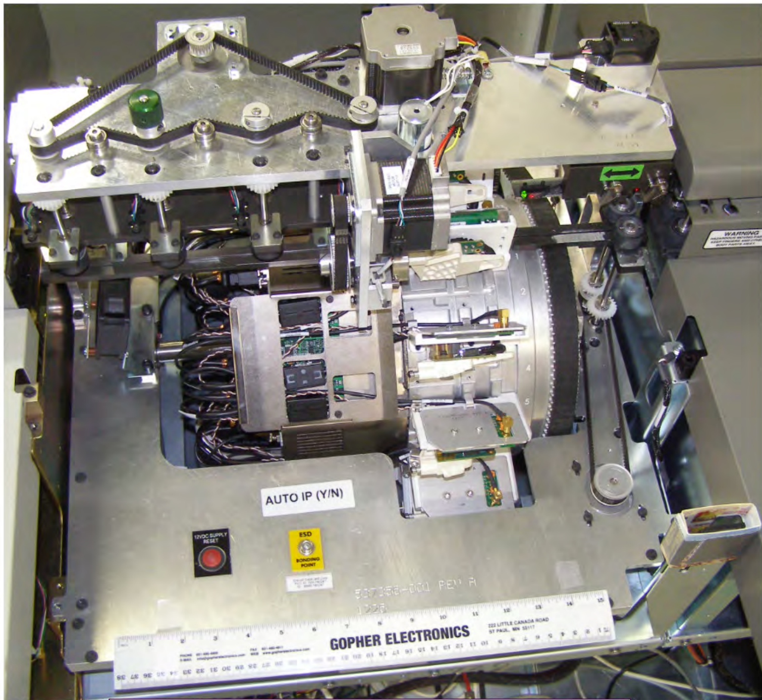
internal / top Barrel Smart Card Module, external skins removed
