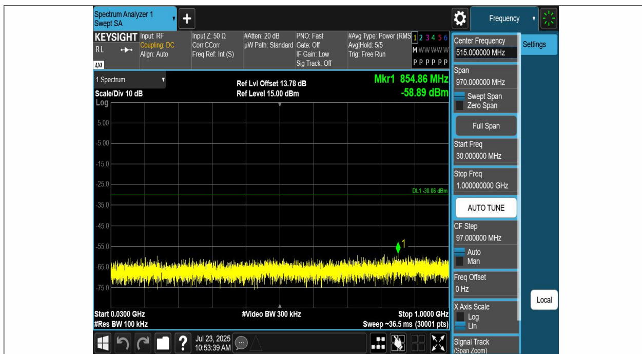
SRD_1M-Ant1-2440-30~1000-PASS
