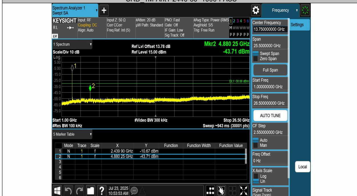
SRD_1M-Ant1-2440-1000~26500-PASS
