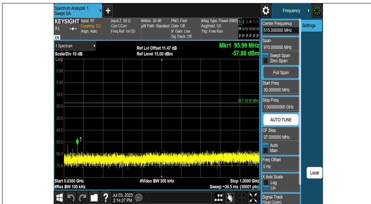
SRD_2M-Ant1-2480-30~1000-PASS
