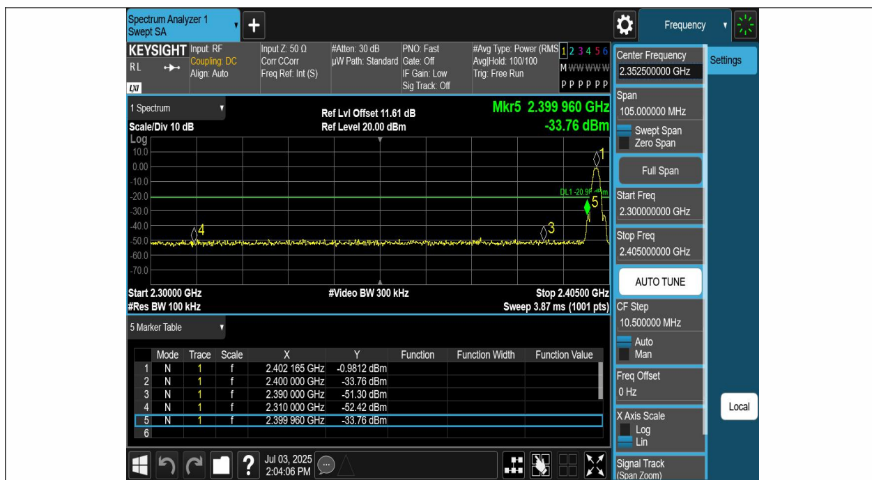
SRD 2M-Ant1-2402-PASS
