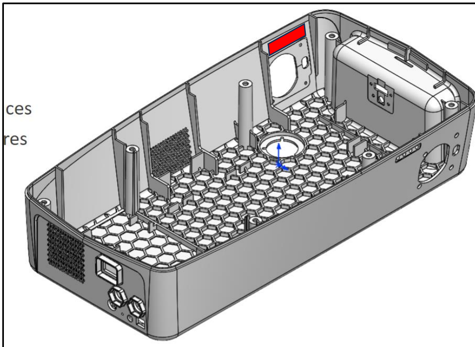
Bottom housing showing placement of antenna.
