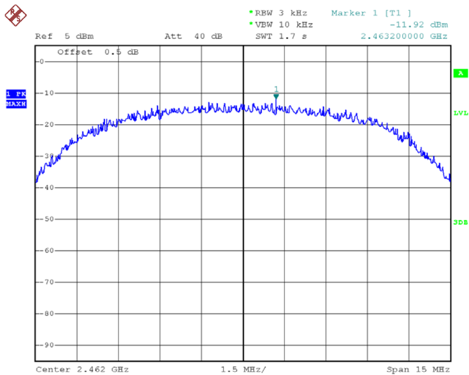
(Plot 2.4 C: Channel = 11 @ 802.11b)
