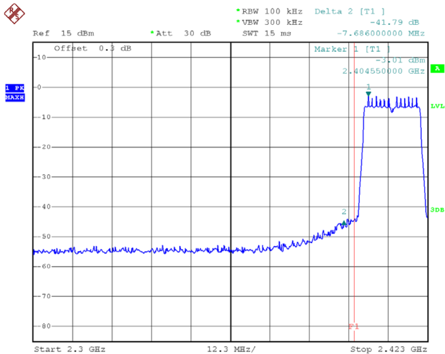
(Plot 2.5.2 C1: Channel =1 2412MHz @ 802.11n-20)
