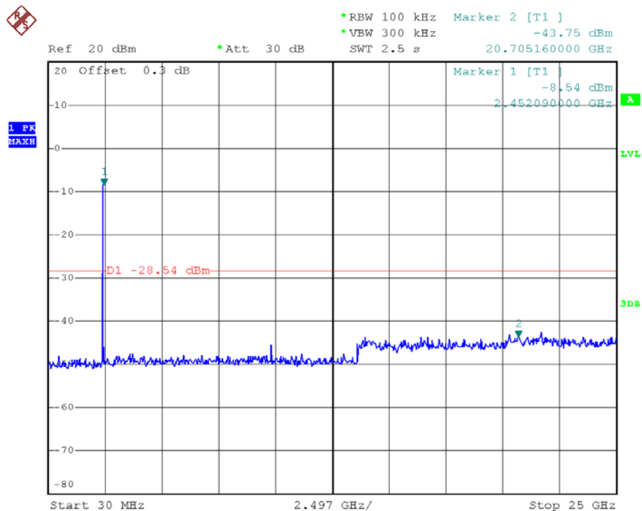
(Plot 2.3 I: Channel = 11, 30MHz to 25GHz@ 802.11n-20)
