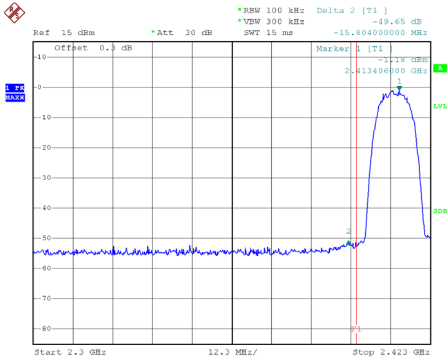
(Plot 2.5.2 A1: Channel =1 2412MHz @ 802.11b)
