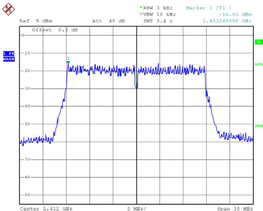
(Plot 2.4 G: Channel = 1 @ 802.11n)
