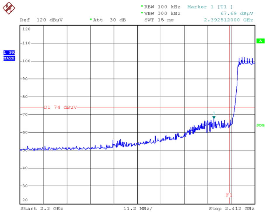
(Plot 2.5.1 D1: Channel = 2 Peak @ 802.11n-40)
