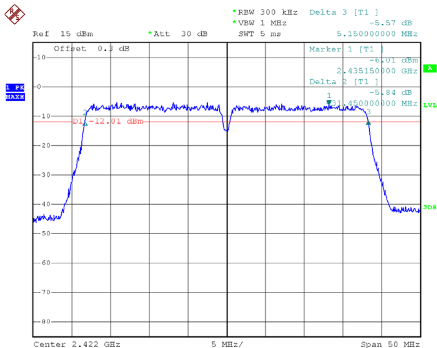
(Plot 2.2 J: Channel 3: 2422MHz @ 802.11n-40)
