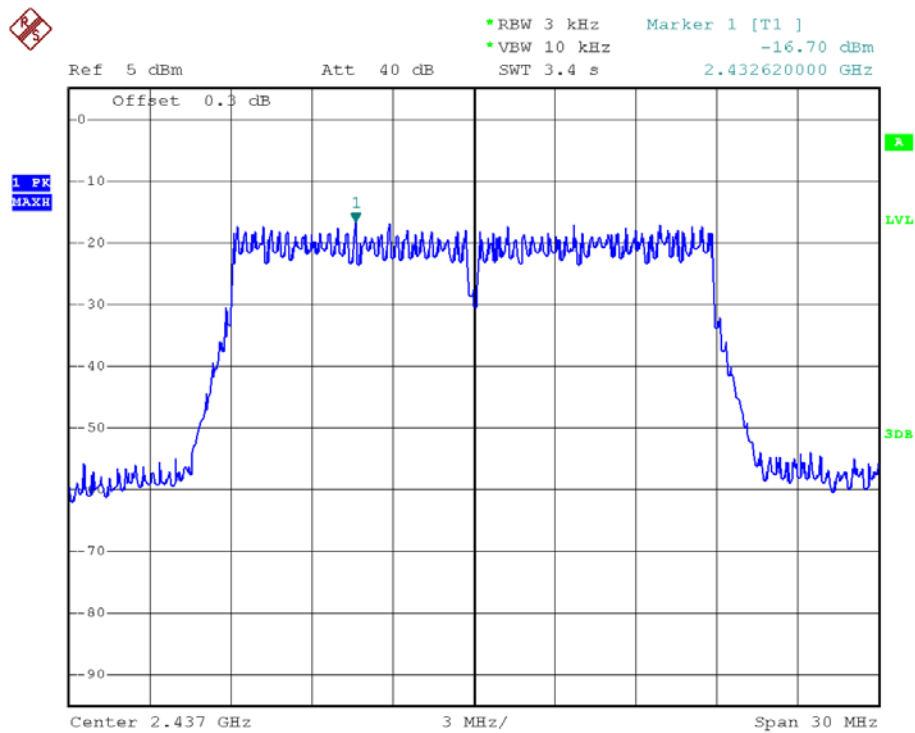
(Plot 2.4 H: Channel = 6 @ 802.11n)
