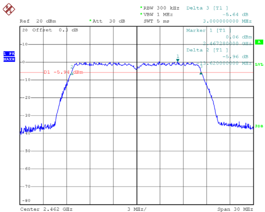
(Plot 2.2 F: Channel 11: 2462MHz @ 802.11g)
