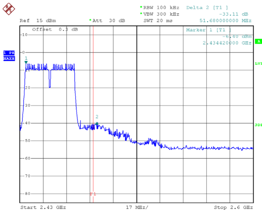
(Plot 2.5.2 D2: Channel =9 2452MHz @ 802.11n-40)
