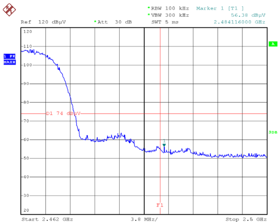
(Plot 2.5.1 A3: Channel = 11 Peak @ 802.11b)
