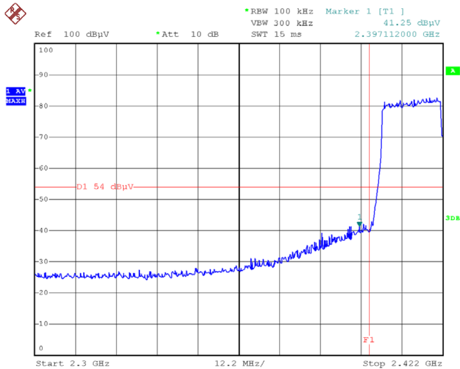
(Plot 2.5.1 D2: Channel = 3 AVG @ 802.11n-40)
