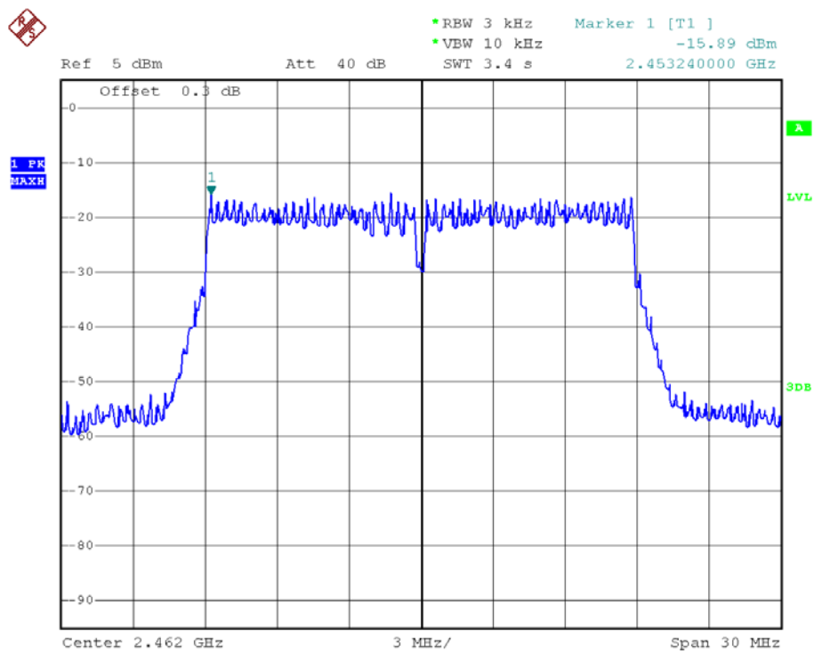
(Plot 2.4 I: Channel = 11 @ 802.11n)
