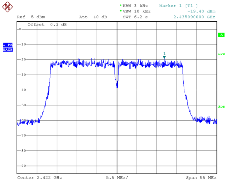
(Plot 2.4 J: Channel = 3 @ 802.11n)
