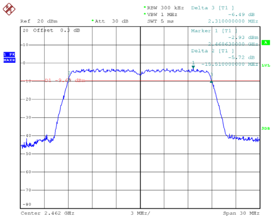
(Plot 2.2 I: Channel 11: 2462MHz @ 802.11n-20)
