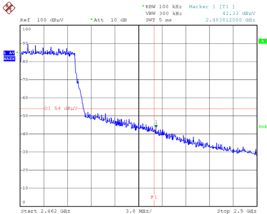
(Plot 2.5.1 C4: Channel = 11 AVG @ 802.11n-20)
