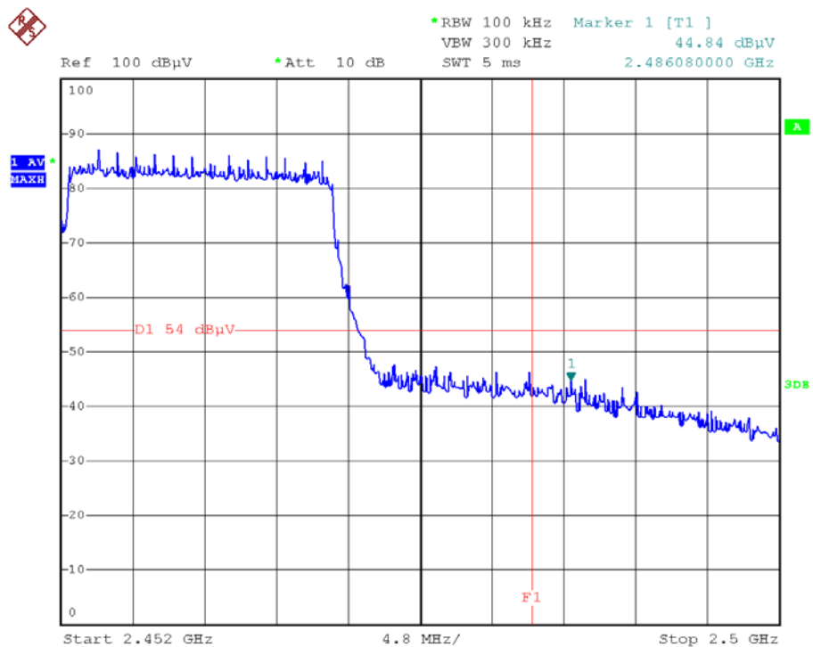
(Plot 2.5.1 D4: Channel = 9 AVG @ 802.11n-40)
