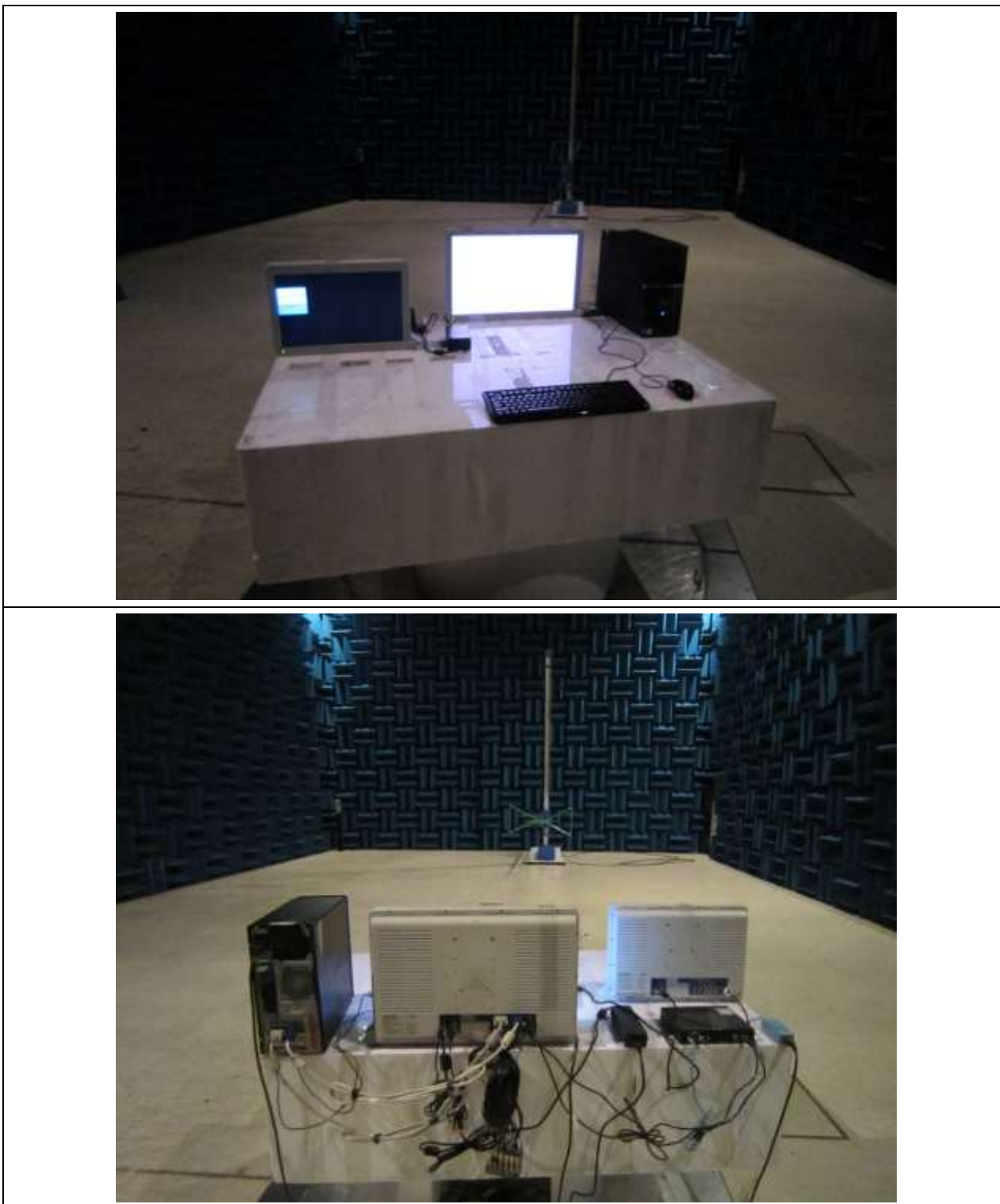
Figure 3. Photo of Radiated Emission Test Setup: DVI Mode
