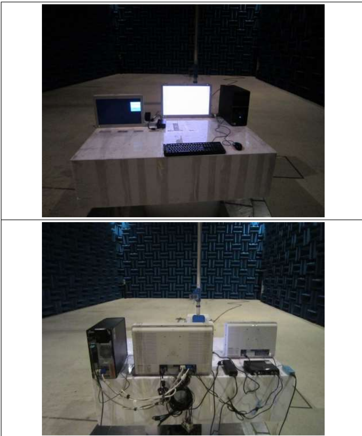
Figure 4. Photo of Radiated Emission Test Setup for Above 1GHz: DVI Mode
