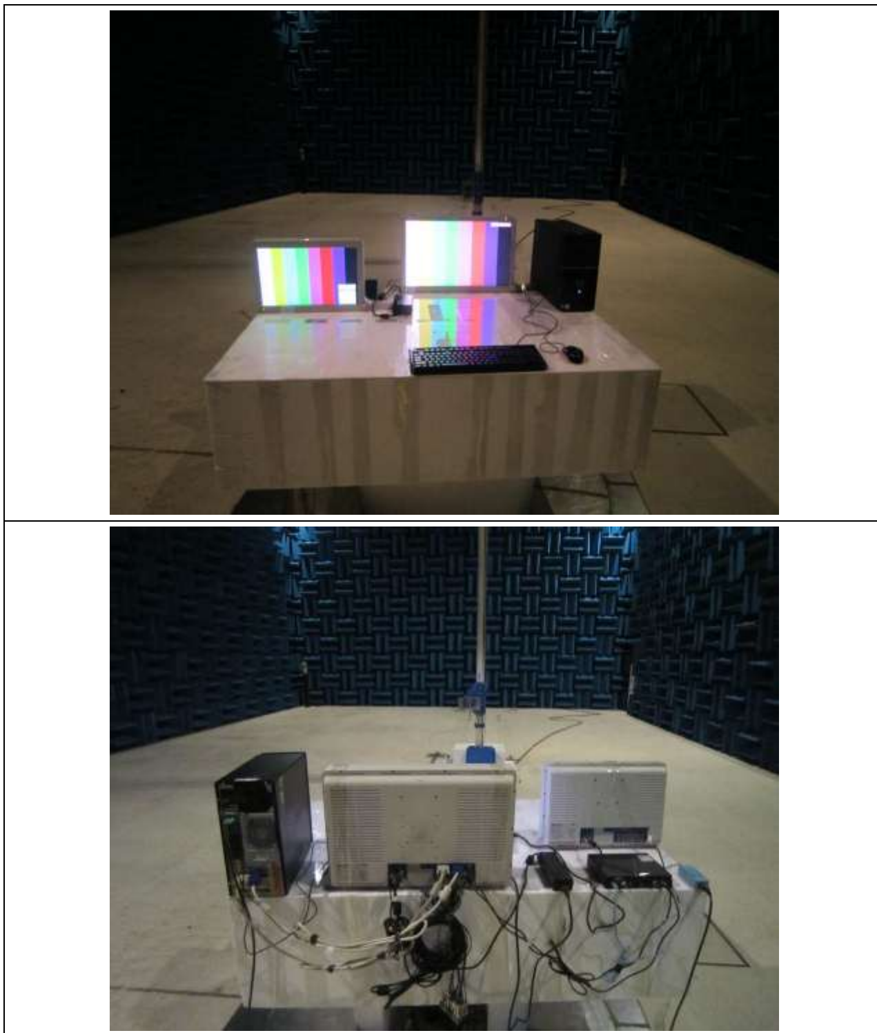
Figure 6. Radiated Emission Test Setup for Above 1GHz: SDI Mode
