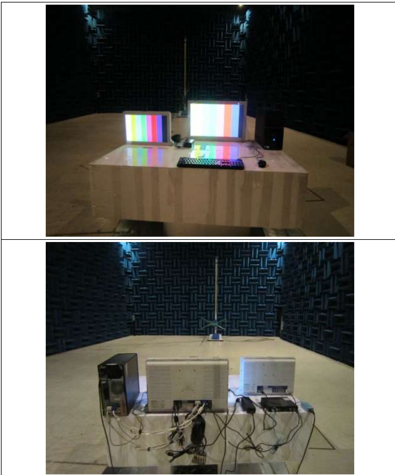
Figure 5. Radiated Emission Test Setup: SDI Mode
