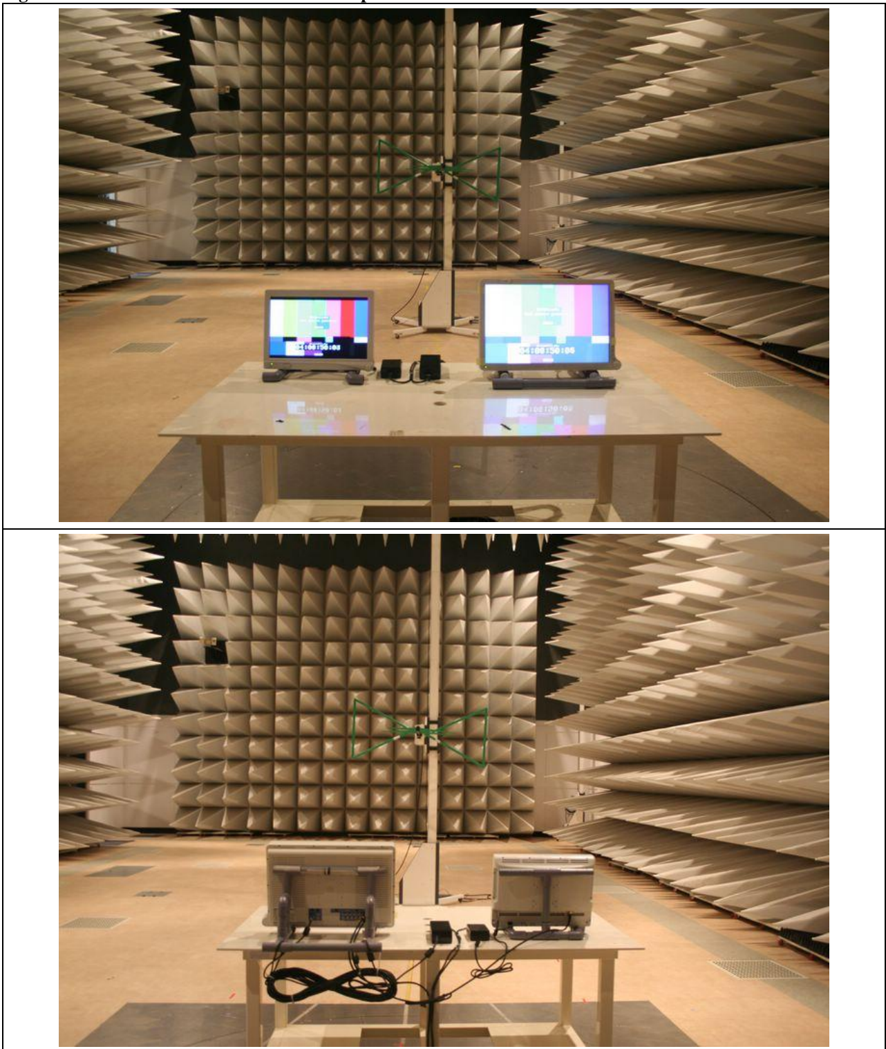
Figure 4. Photo of Radiated emission test setup for SDI In/Out Mode
