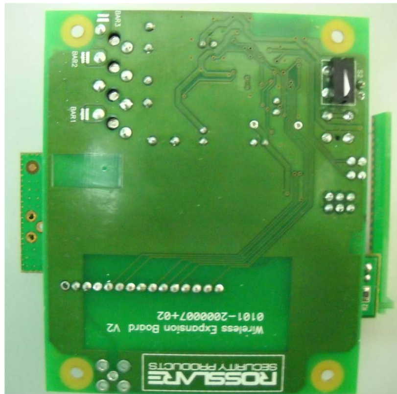
Photograph No.4 XR-16AG PCBs second side view
