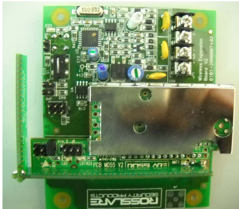
Photograph No.3 XR-16AG PCBs top view
