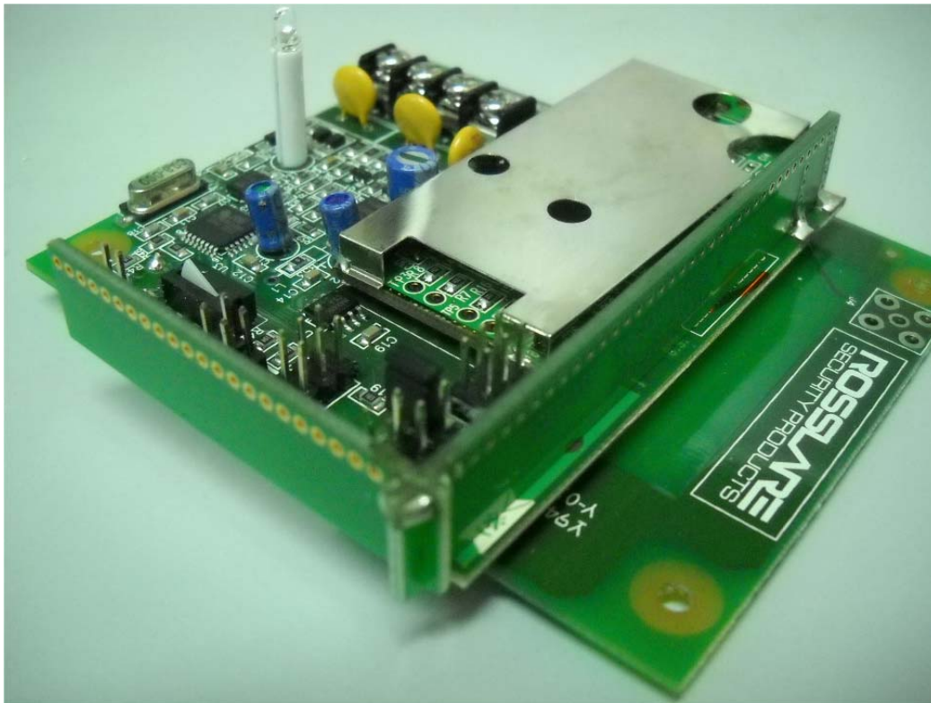
Photograph No.5 XR-16AG PCBs side view
