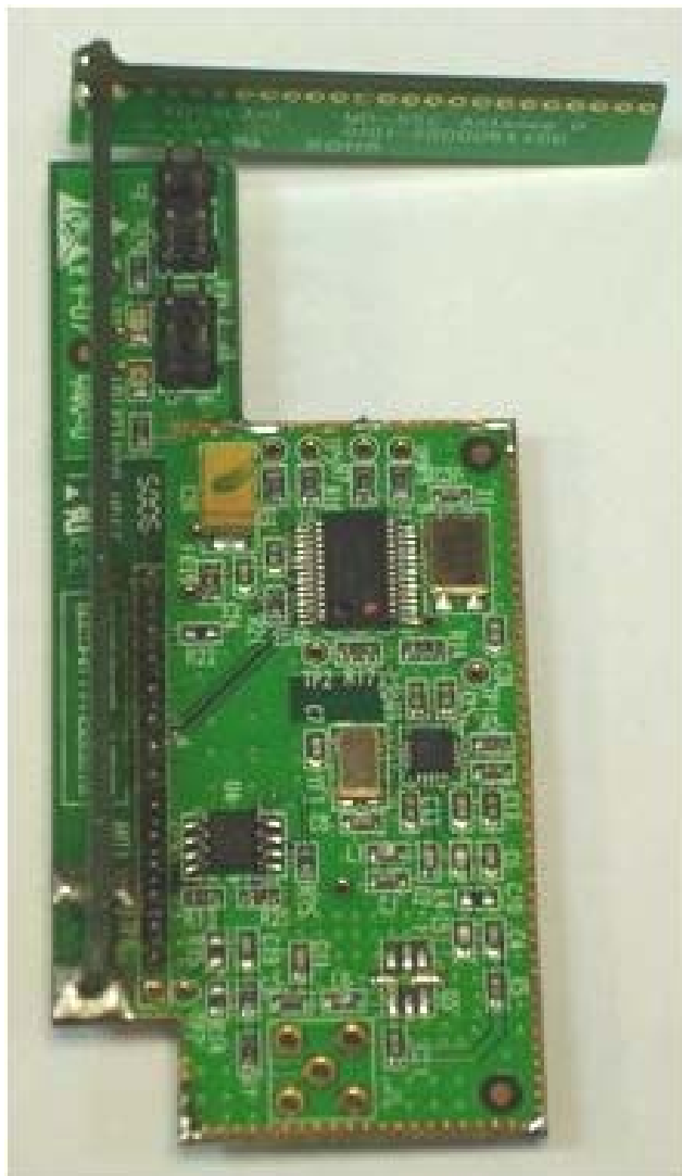
Photograph No.8 RF PCB without shielding
