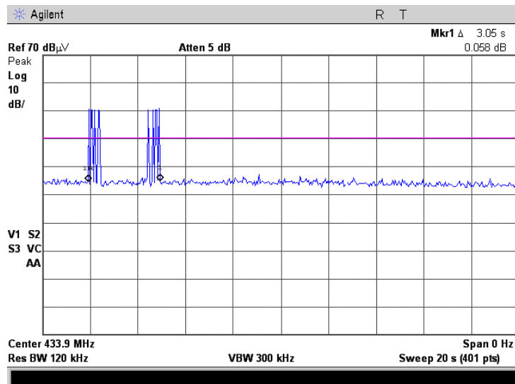
Plot 7.1.2 Transmitter shut down test result
