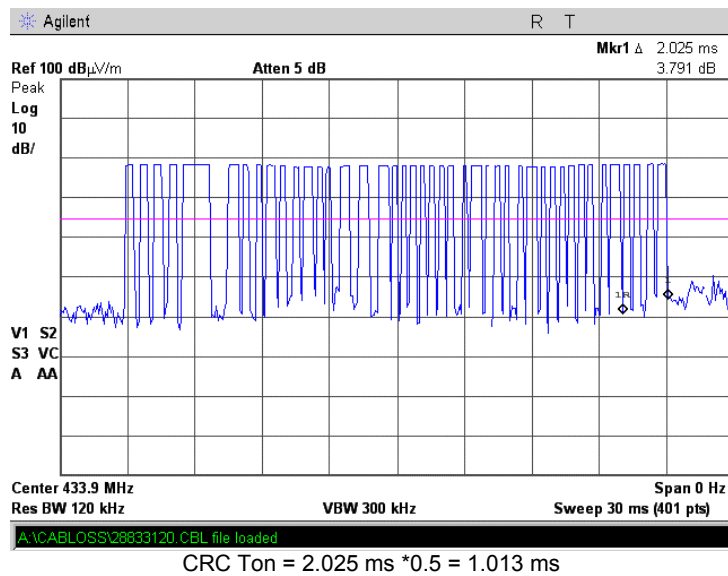
Plot 7.2.21 Transmission pulse duration
