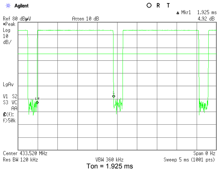
Plot 7.2.16 Transmission pulse period, 433.52 MHz
