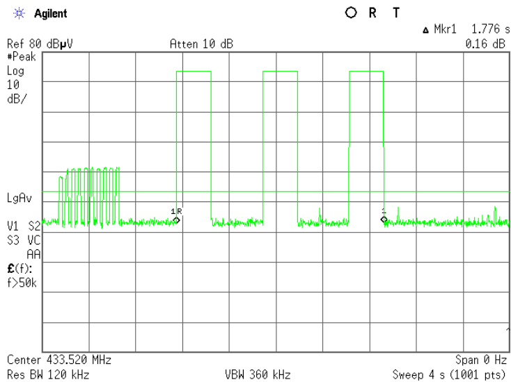
Plot 7.2.18 Transmission train duration, 433.52 MHz
