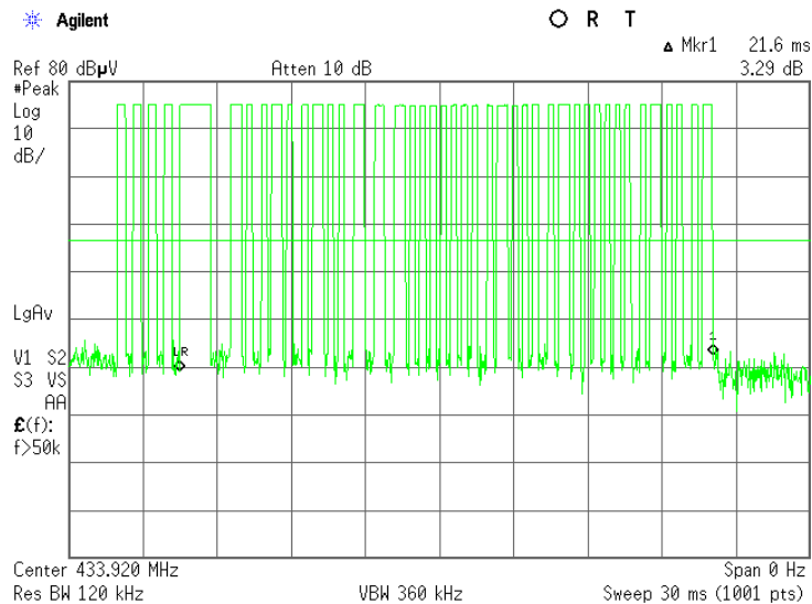
Plot 7.3.17 Transmission burst duration, 433.92 MHz
