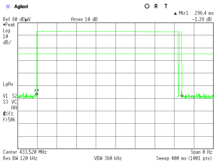
Plot 7.2.17 Transmission burst duration, 433.52 MHz
