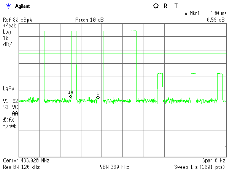
Plot 7.3.19 Transmission burst period, 433.92 MHz
