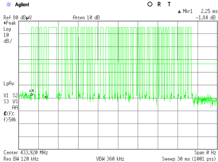
Plot 7.3.16 Transmission burst duration, 433.92 MHz
