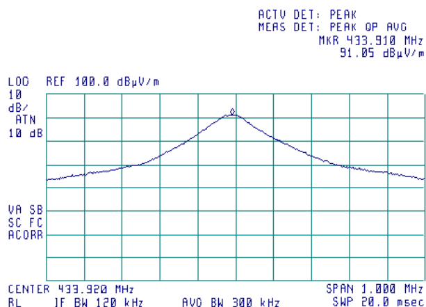
Plot 7.3.6 Radiated emission measurements at the fundamental frequency
