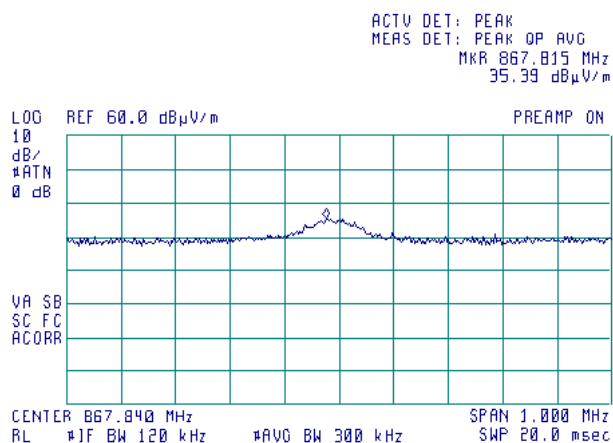
Plot 7.3.14 Radiated emission measurements at the third harmonic frequency
