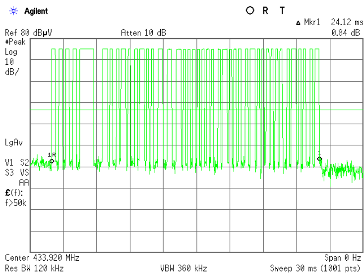
Plot 7.3.18 Transmission burst duration, 433.92 MHz
