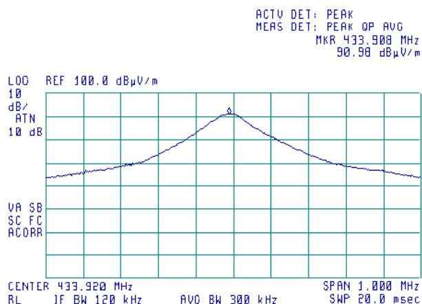
Plot 7.3.4 Radiated emission measurements at the fundamental frequency
