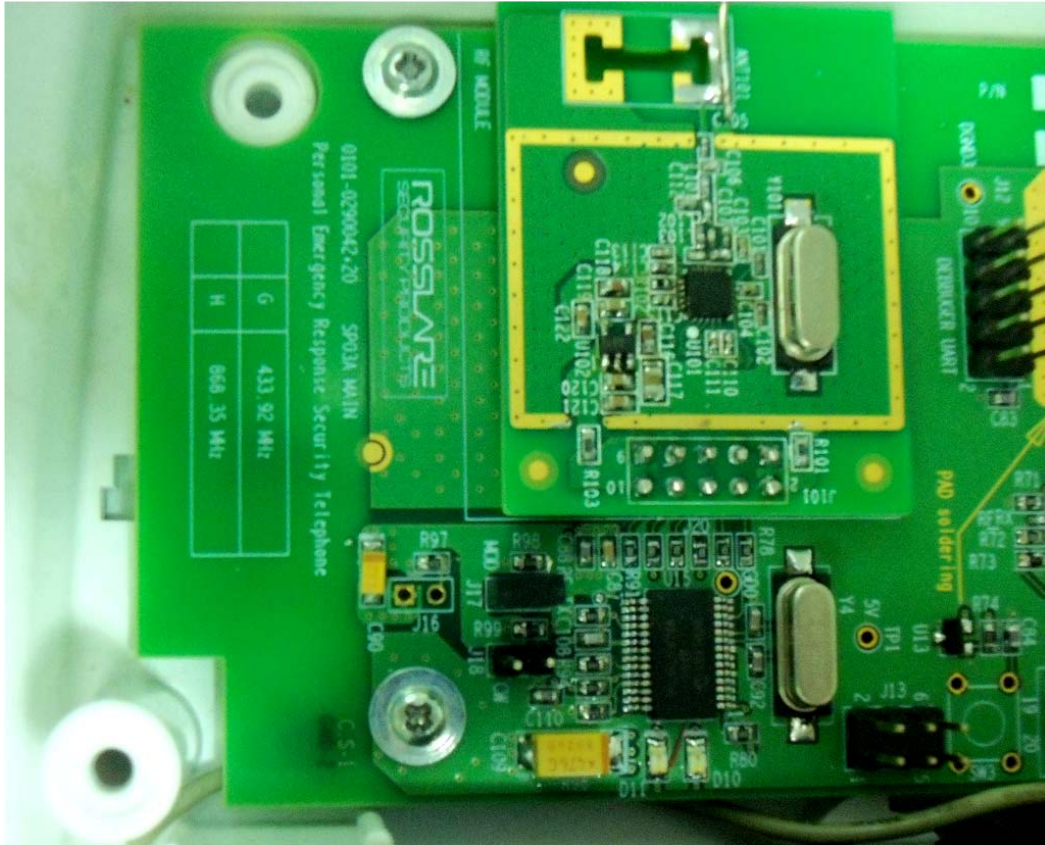
Photograph No.5 Main PCB with RF PCB close view
