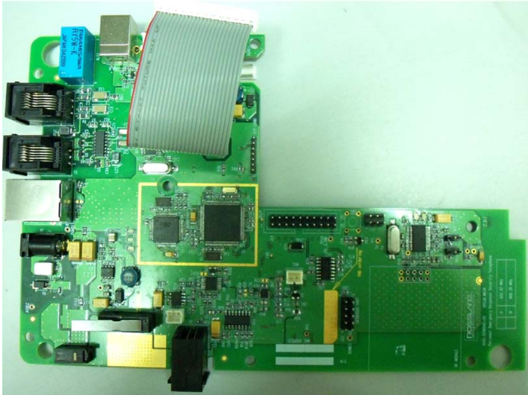
Photograph No.6 Main PCB with RF PCB removed
