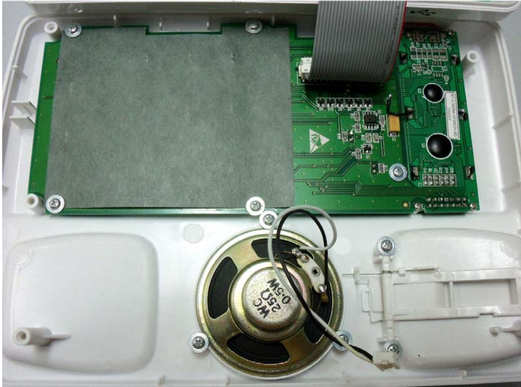
Photograph No.2 Wireless Elderly Assist SP-03V2G internal view (cover)
