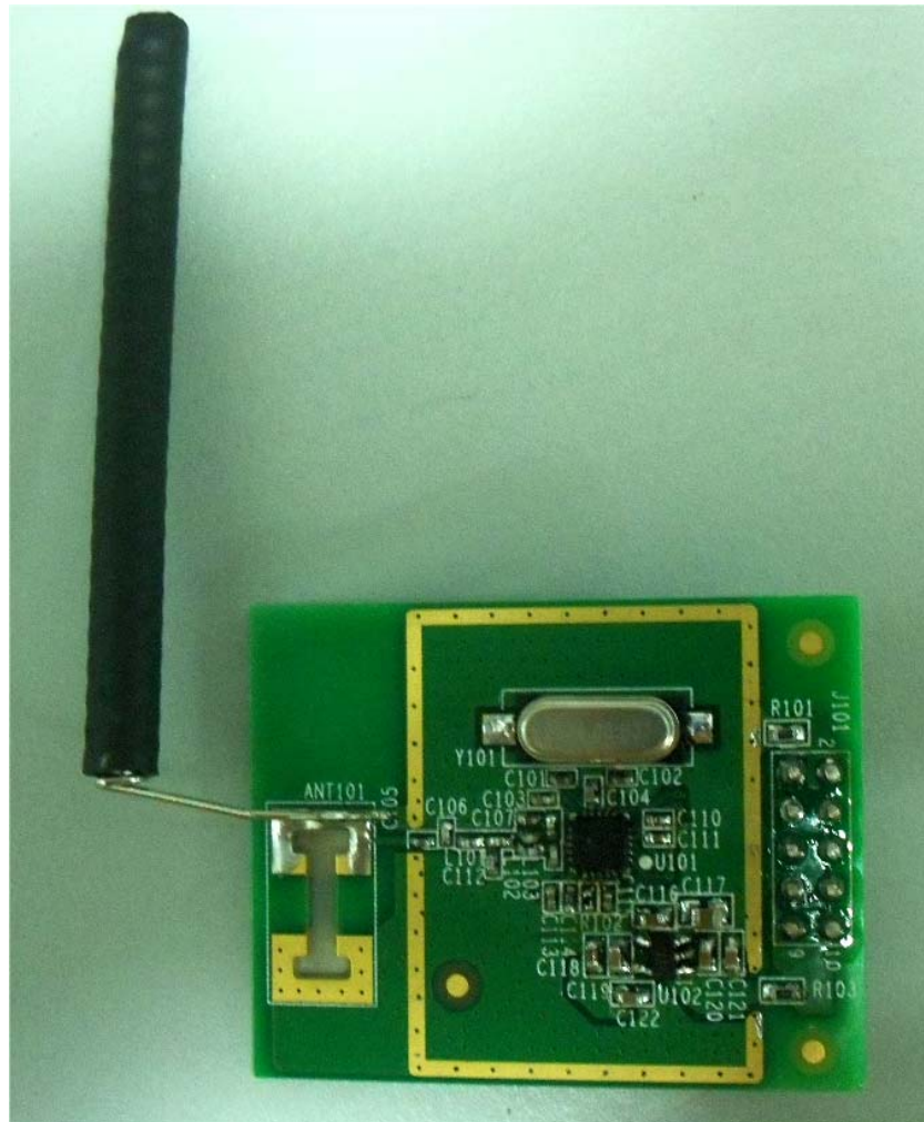
Photograph No.9 RF PCB front view
