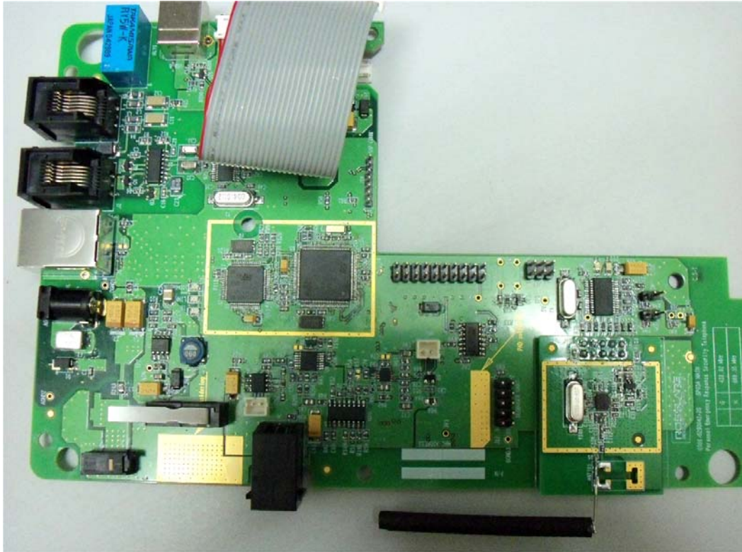
Photograph No.4 Main PCB front view
