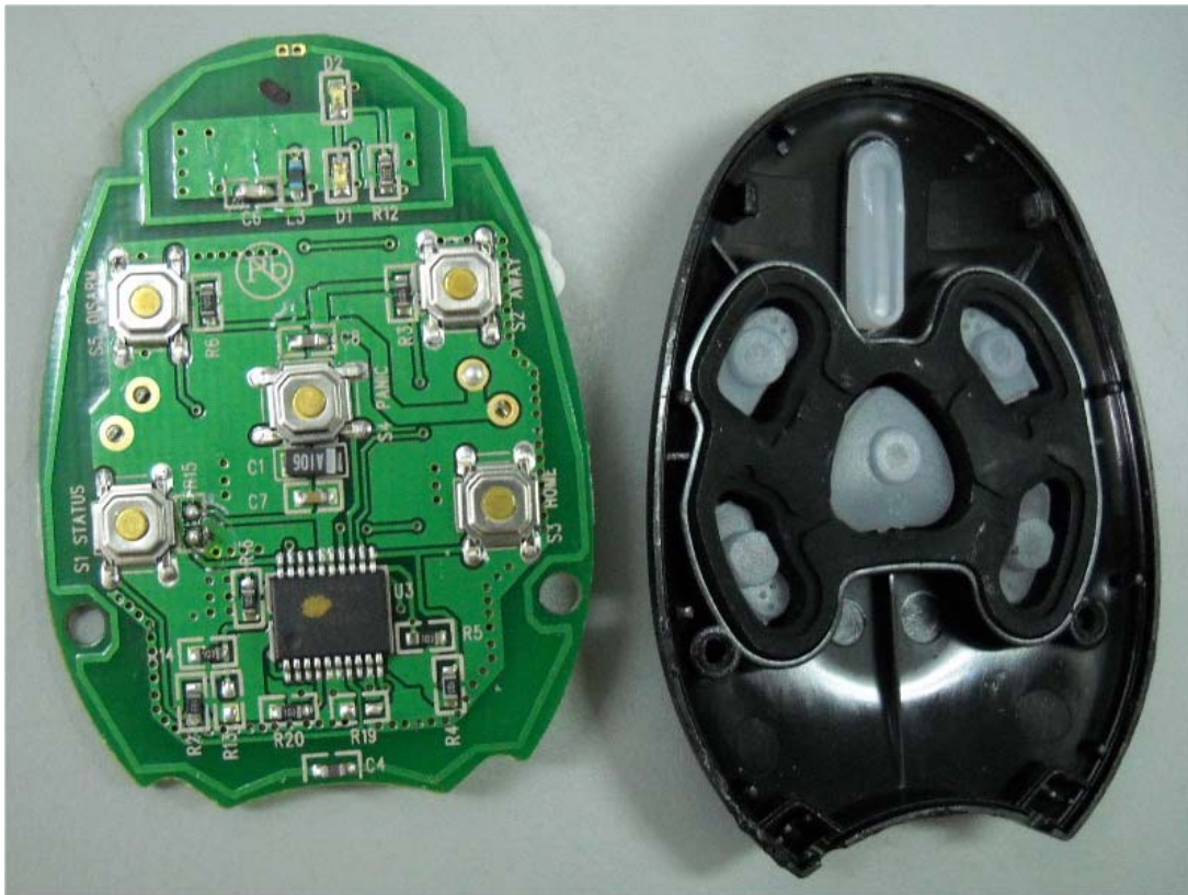
Photograph No.4 SA-33G remote control internal view
