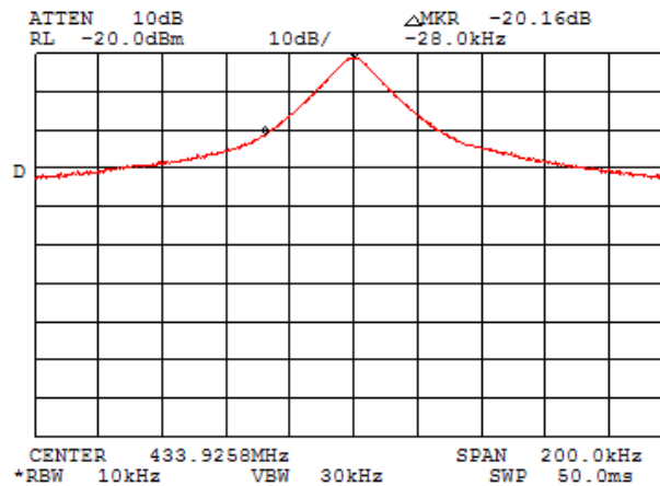
Plot 7.3.1 Occupied bandwidth test result
