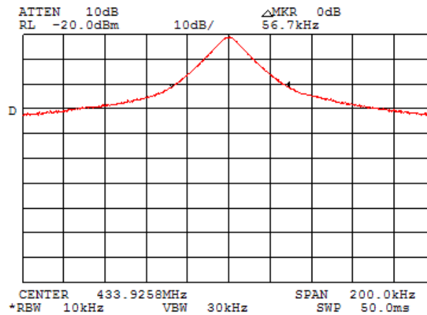
Plot 7.3.2 Occupied bandwidth test result
