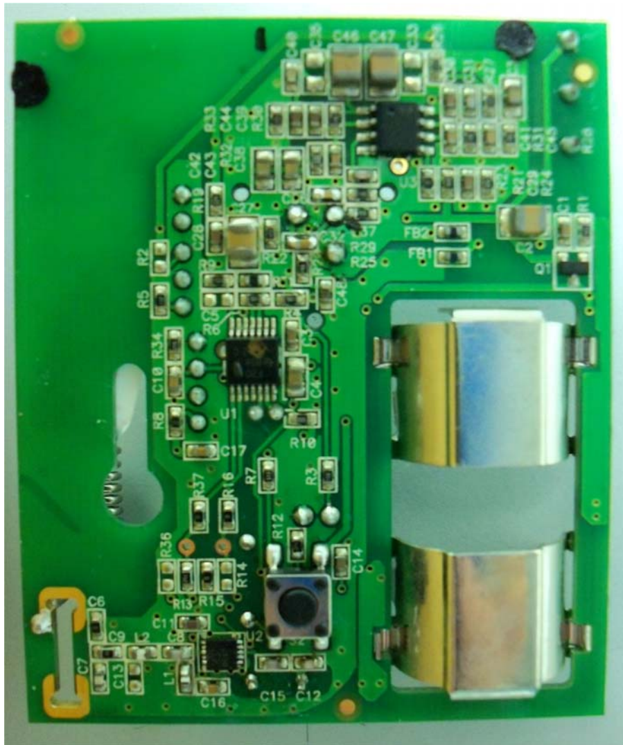
Photograph No.5 PCB second side view
