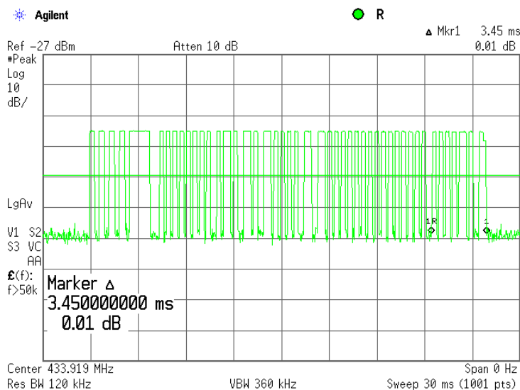
Plot 7.2.22 Transmission burst duration
