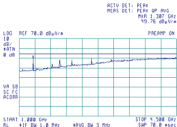
Plot 7.2.7 Radiated emission measurements from 1000 to 4500 MHz
