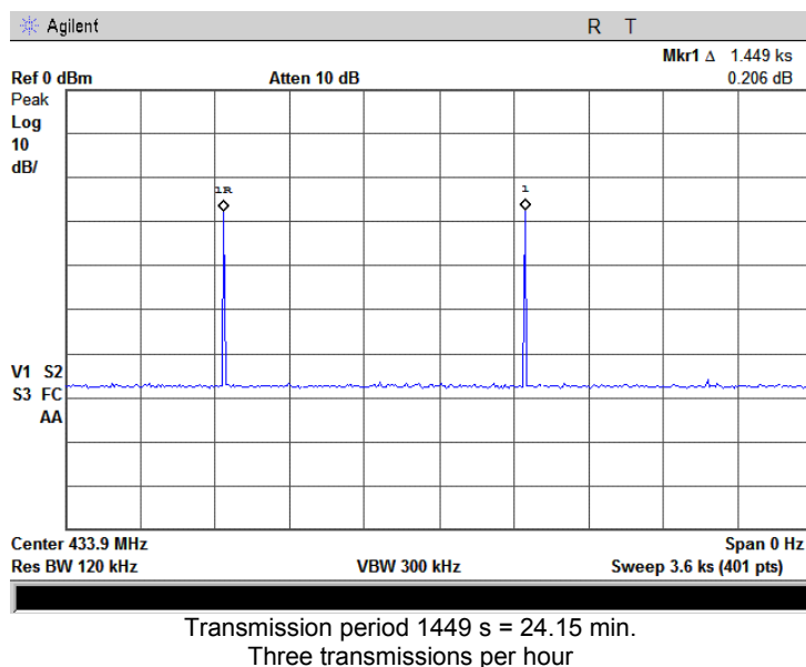
Plot 7.1.3 Polling / supervision transmission duration
