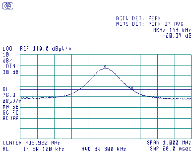
Plot 7.3.2 Occupied bandwidth test result
