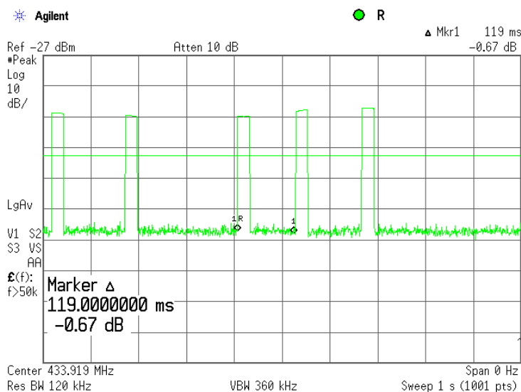
Plot 7.2.23 Transmission burst period
