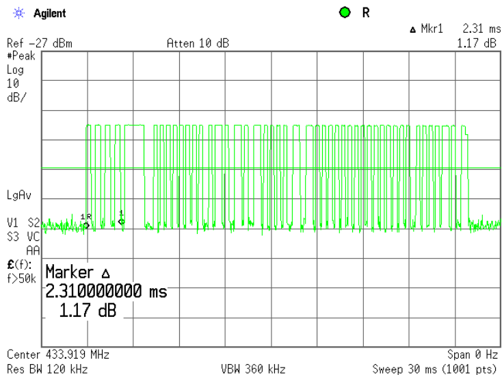
Plot 7.2.20 Transmission burst duration
