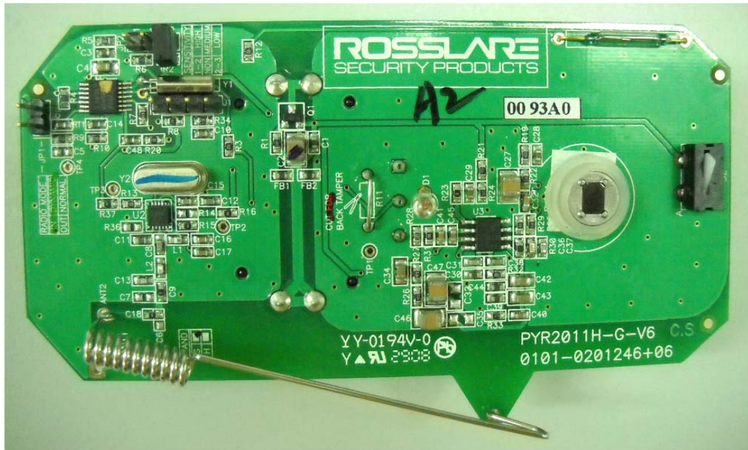
Photograph No.3 PCB top view
