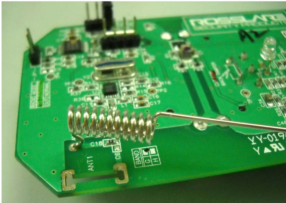
Photograph No.5 Antenna close view
