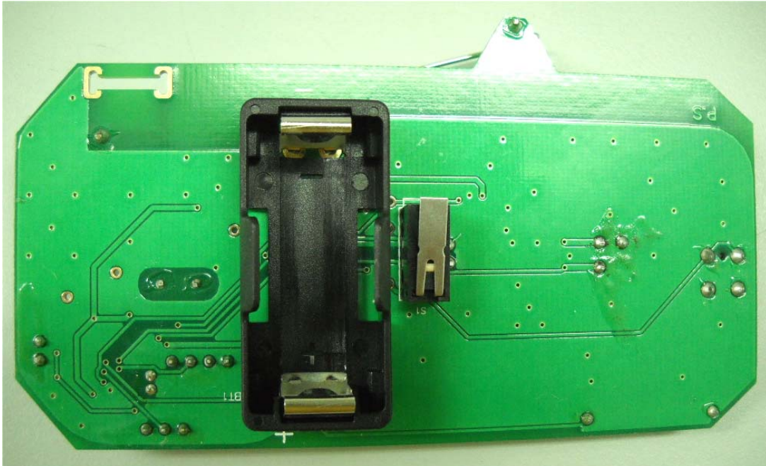
Photograph No.4 PCB second side view
