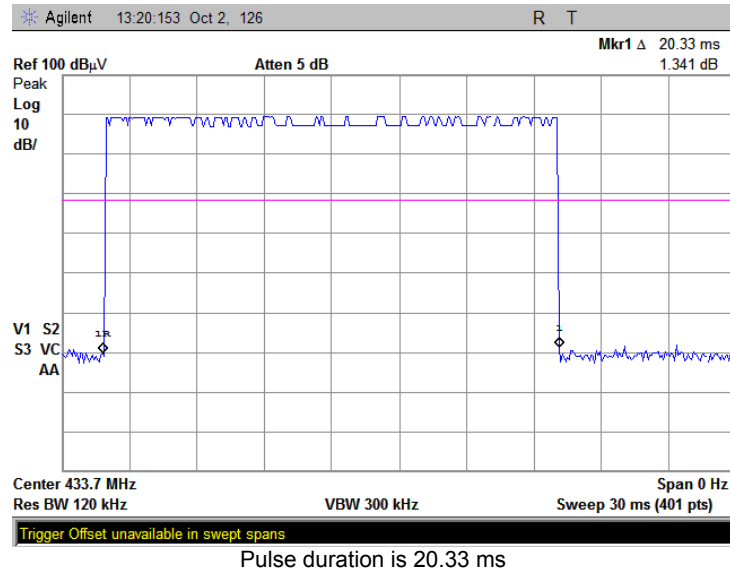
Plot 7.1.6 Polling / supervision transmission duration
