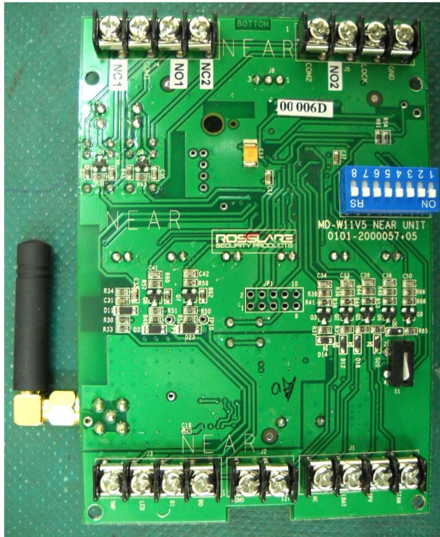
Photograph No.4 PCB second side view
