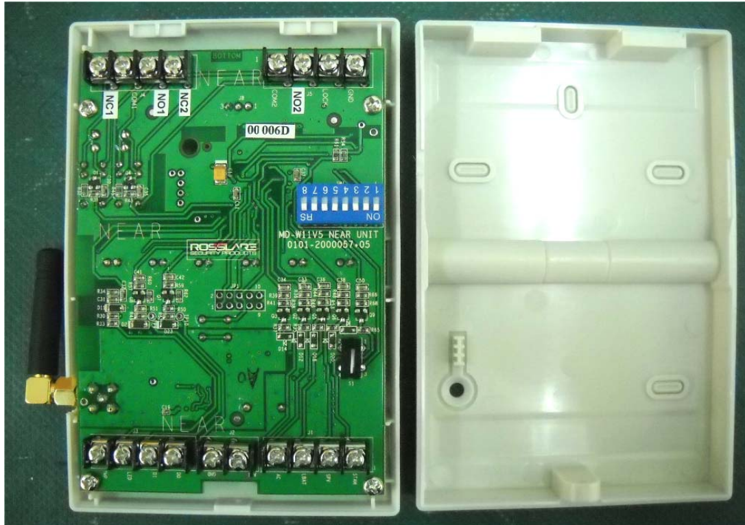
Photograph No.1 MD-W11NGR Near unit internal view
