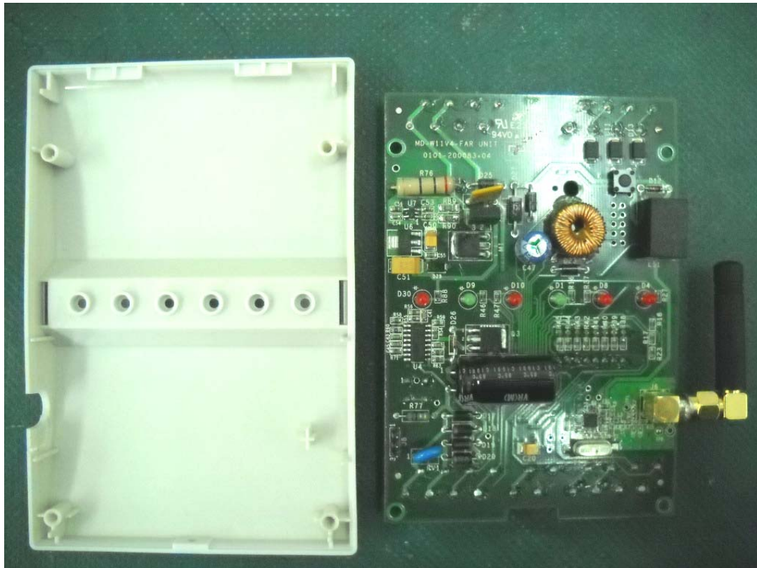
Photograph No.2 MD-W11FGR Far unit internal view
