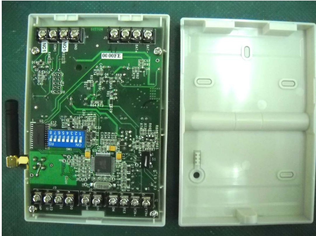
Photograph No.1 MD-W11FGR Far unit internal view
